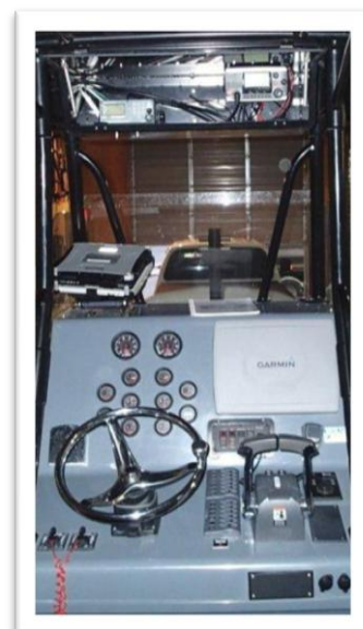
Figure 4.29.3 Console & Transponder
