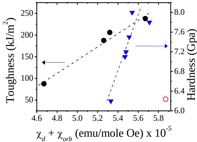
Figure 3.3: Toughness (●) and hardness (▼) properties for Zr and ZrHf-based BMGs are plotted versus \chi_d + \chi_{orb} from Table 1 showing an approximately linear correlation. The outlier of the trend seen here is from Zr_{56}Co_{28}Al_{16} due to enhanced \chi_{orb} and is noted with a different symbol (○).
