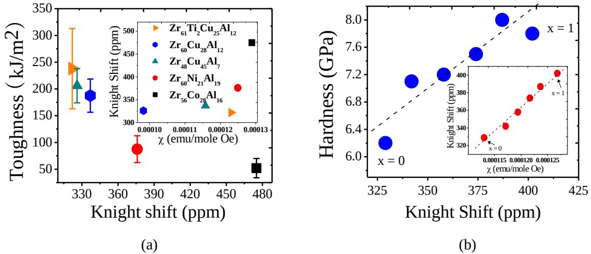
Figure 3.2: (a) Toughness ( \text{kJ/m}^2 ) properties are plotted as a function of Knight shift K_{\text{iso}} for Zr-based BMGs demonstrating a direct correlation between mechanical properties and local electronic structure. (b) Hardness (GPa) properties of ZrHf-based BMGs are plotted versus the Knight shift K_{\text{iso}} showing a
