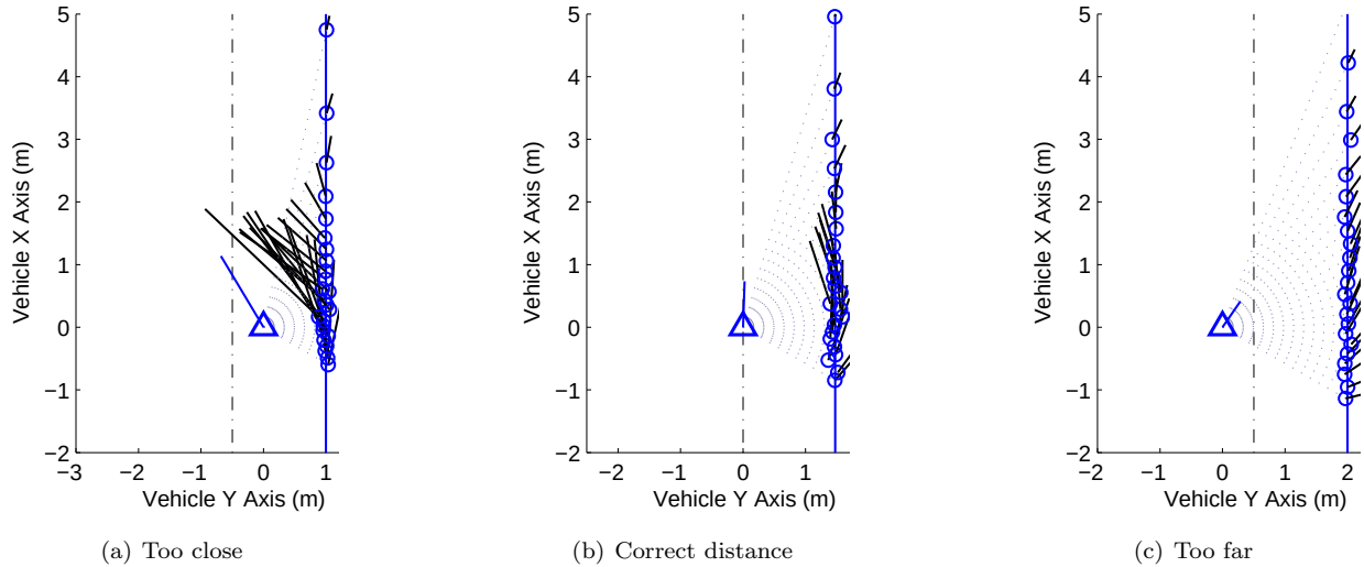
Figure 3. The guidance algorithm generates a velocity vector from the average of vectors generated for each range measurement. Along a section of straight wall, the algorithm gives corrections to keep the vehicle a desired distance from the wall, which is indicated by a dotted line. The wall is shown by a solid vertical line, with individual range measurements shown by circles. Individual velocity increments are indicated by a line showing the magnitude and direction at each measurement point. The total commanded velocity is shown by a line emanating from the vehicle, which is represented by a triangle.
