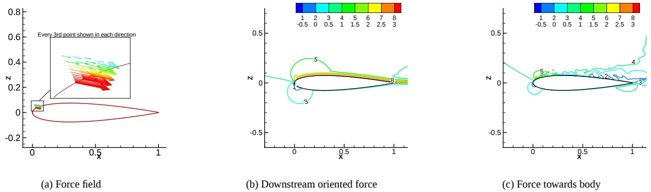
Figure 4. STEADY FORCE AND EFFECT ON u -VELOCITY WITH PHENOMENOLOGICAL MODEL
