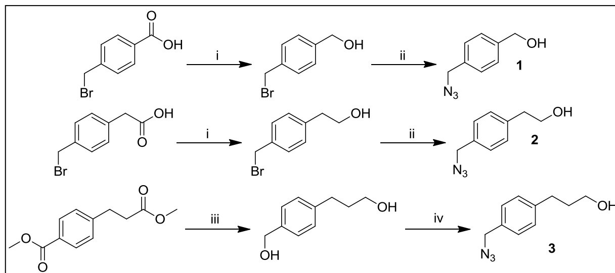
Scheme 3. Azido-alcohol precursors preparation i) \text{BH}_3\cdot\text{THF} , THF; 0 °C to RT; 15 h ii) \text{NaN}_3 , DMSO; 15 h iii) \text{LiAlH}_4 , THF; 0 °C to RT; 15 h iv) \text{SOCl}_2 , DIPEA, DCM; 1h. Silica flash column purification and ^1\text{H} -NMR characterization were performed for each precursor.
