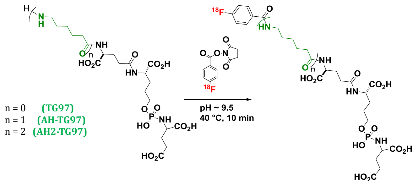
Scheme 2. [ ^{18}\text{F} ]SFB to the PSMA inhibitor lead analogues
