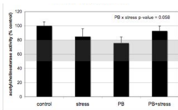
Figure 14. Acetylcholinesterase activity was inhibited to within therapeutic levels in the PB-treated muscle at 0-d post-treatment. Data are means ( n = 4 ) \pm s.e.
