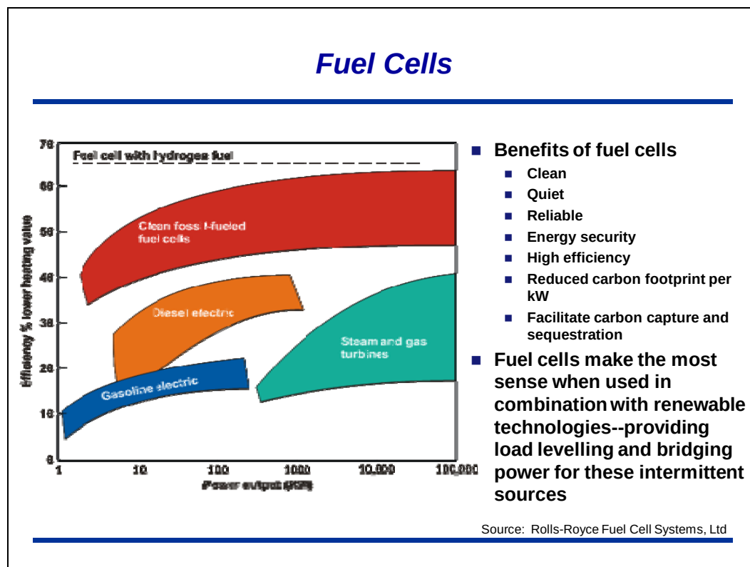
Figure 4-4. Fuel Cell Technology Comparison: Efficiency versus Power Output.
