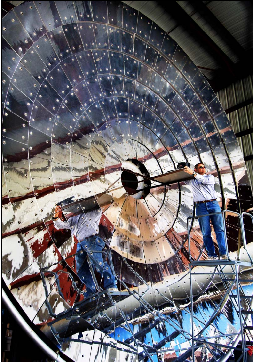
Figure 4-7. Sandia Researcher Rich Diver Checks the Solar Furnace which will be the Initial Source of Concentrated Solar Heat. (Eventually parabolic dishes will provide the thermal energy.) [Photo by Randy Montoya]
