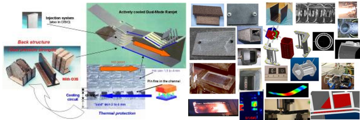
Figure 18: The monobloc CMC technology : PTAH-SOCAR.
