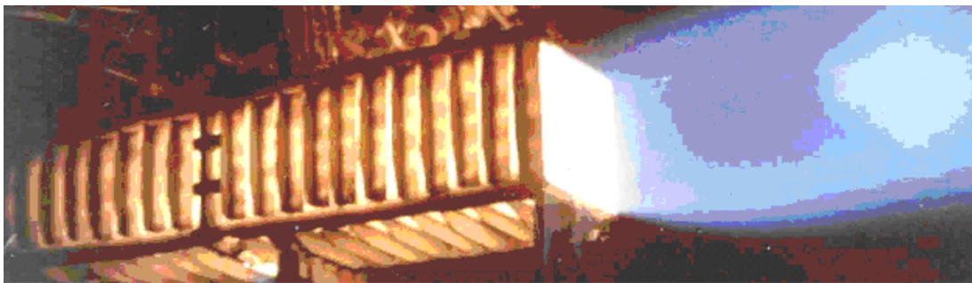
Figure 13: Massive Niobium scramjet combustor under Mach 6 flight conditions testing (MAI).
