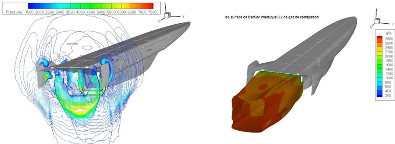
Figure 10: Study of the interaction between propulsive jet and fins.
