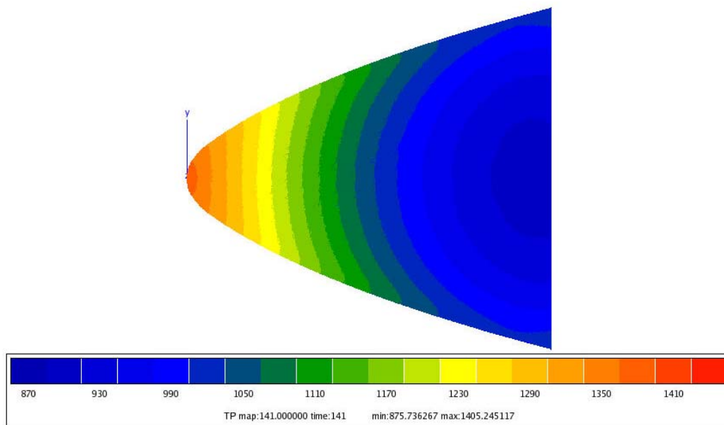
Figure 17: Temperature profile on forebody nose.
