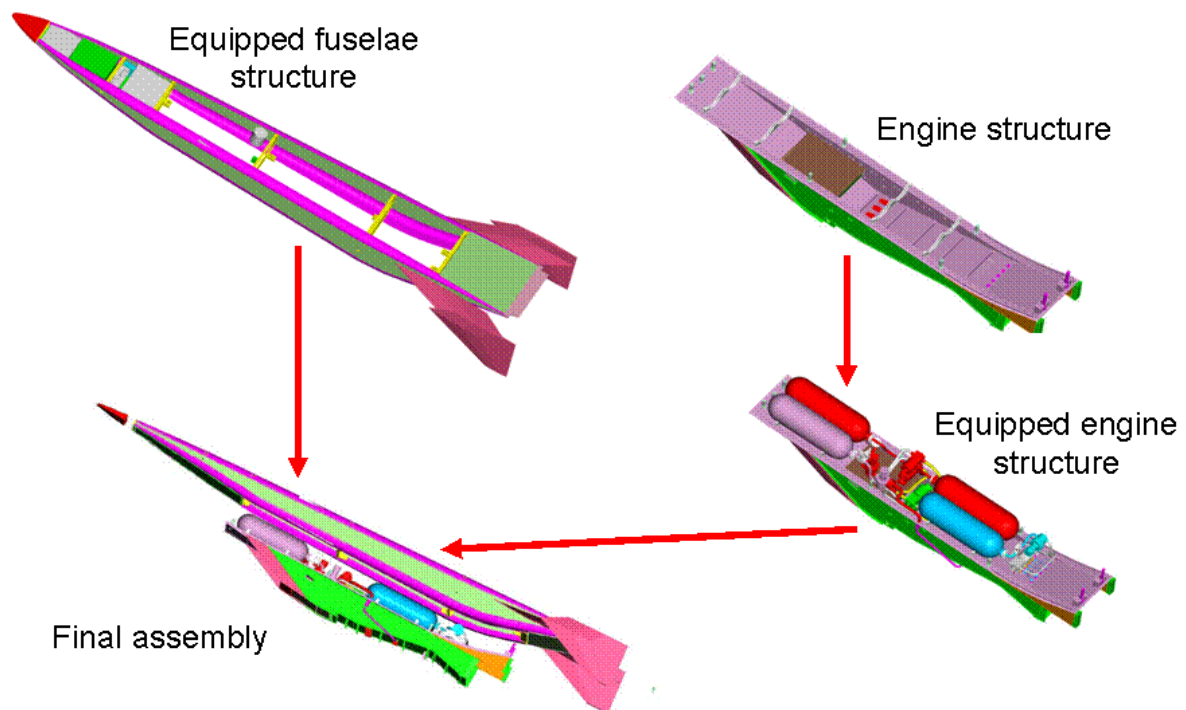
Figure 14: General integration process.
