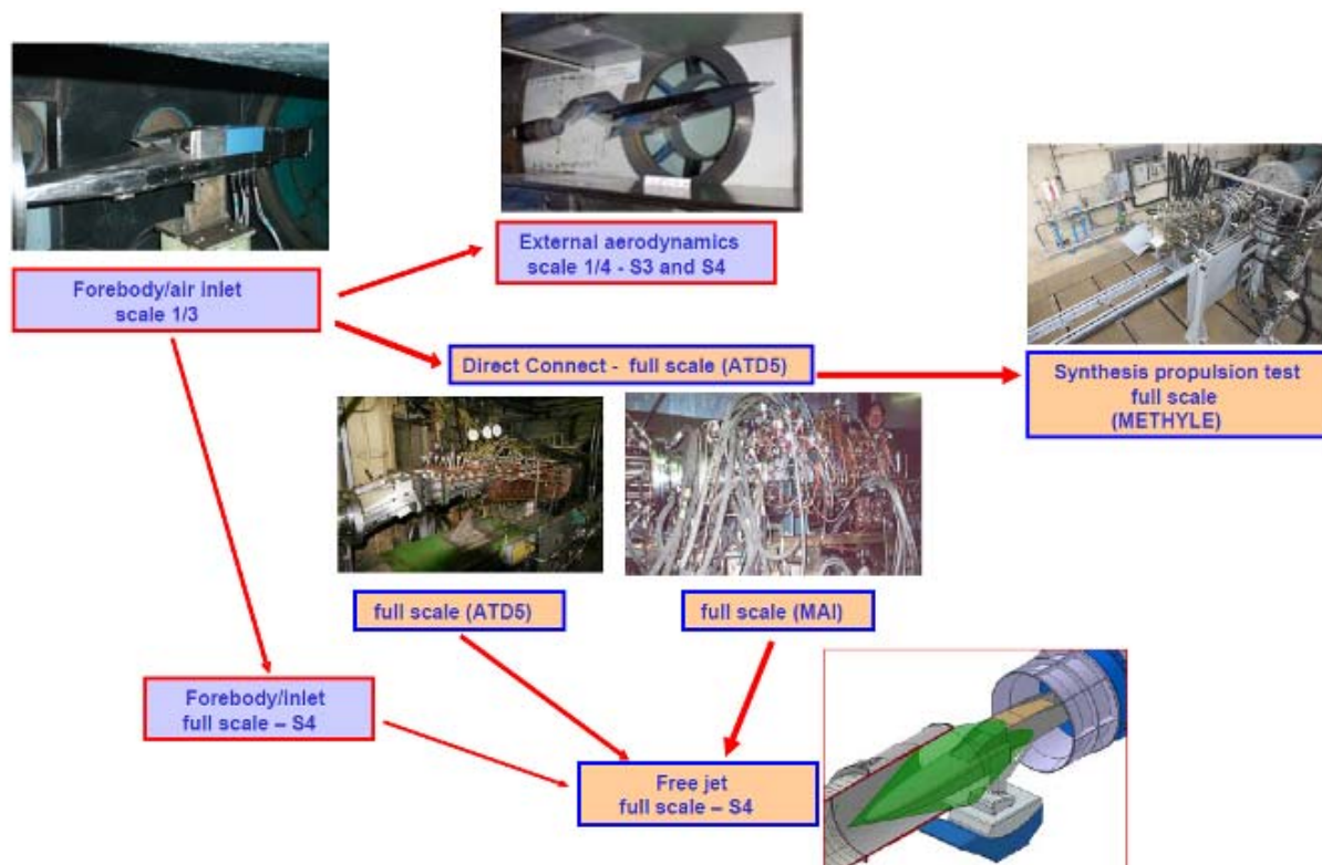
Figure 18: Ground testing logic.
