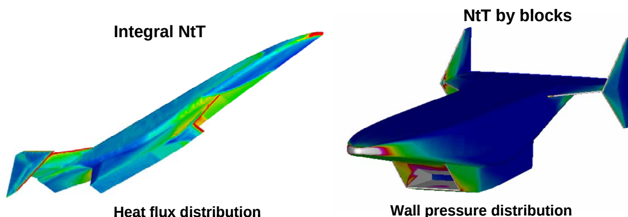
Figure 13: Examples of Nose-to-Tail computation.
