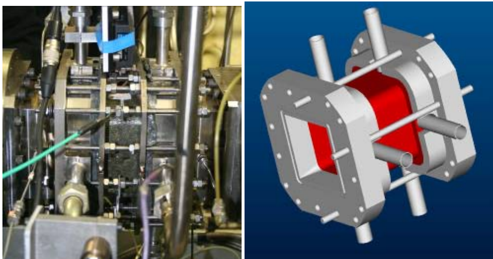
Figure 1: Cooled composite combustion chamber duct (in red) tested at ONERA ATD5.
