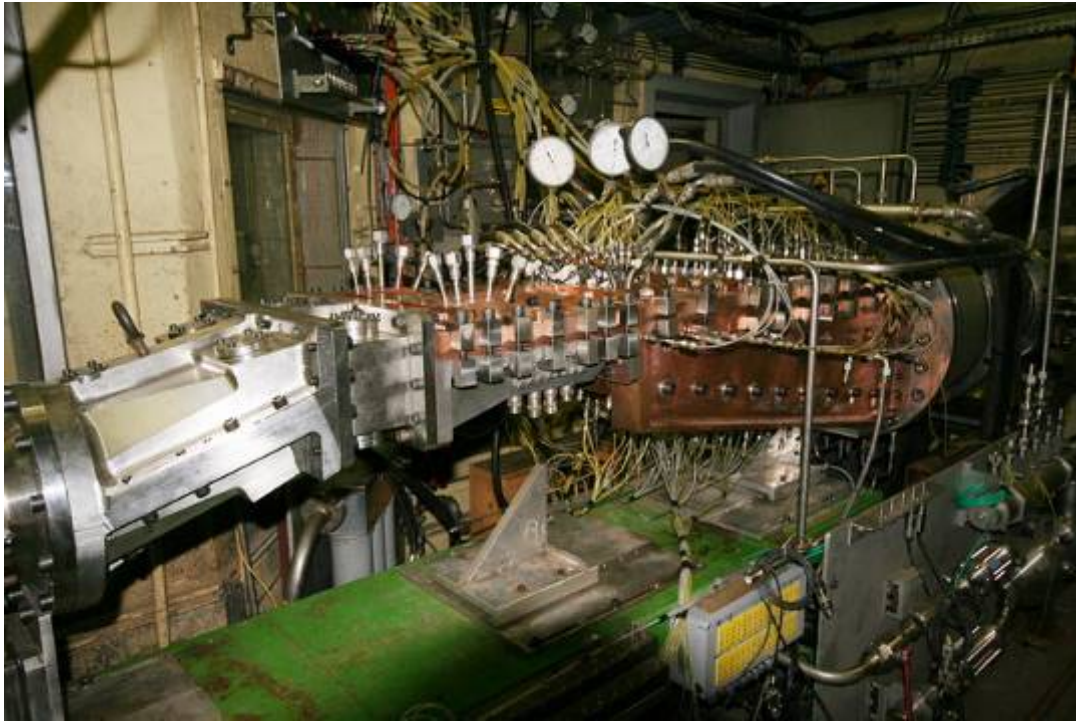
Figure 8: CLEA model under test at ONERA test facility.
