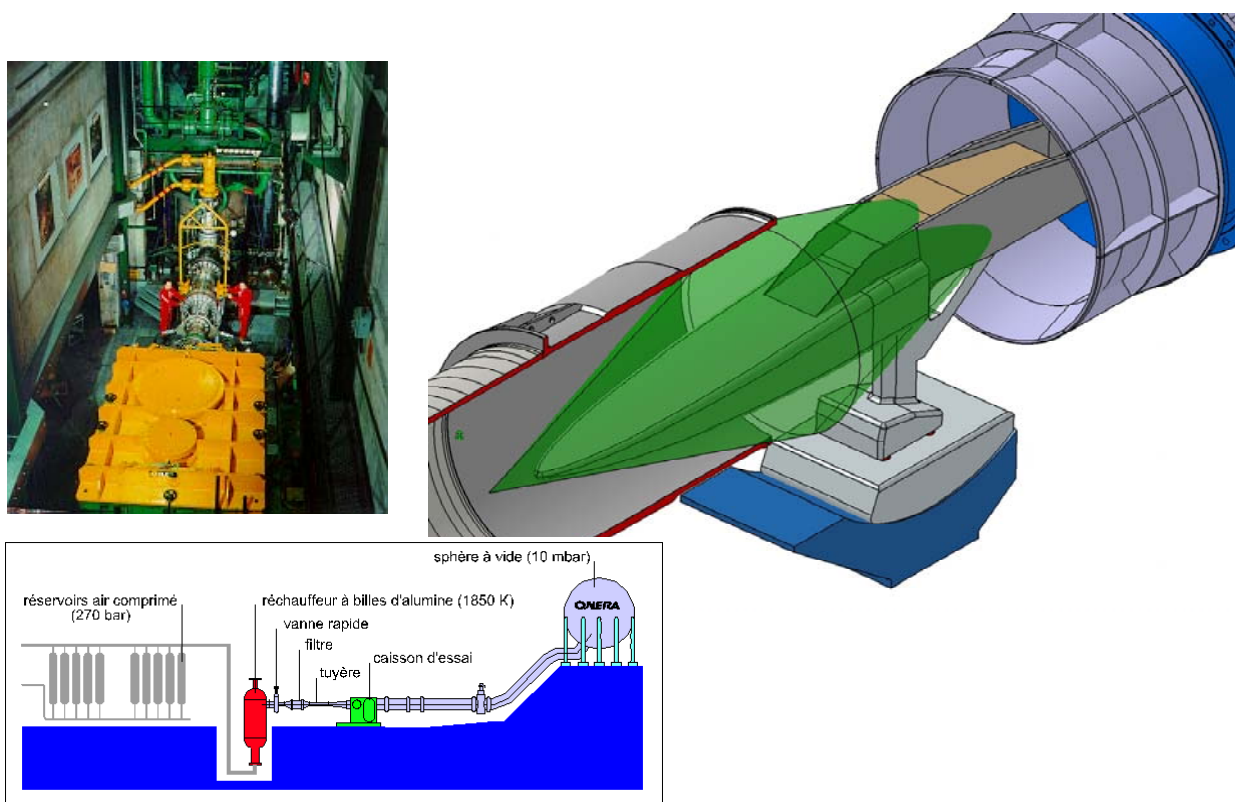
Figure 19: LEA free-jet test installation in S4Ma test facility.
