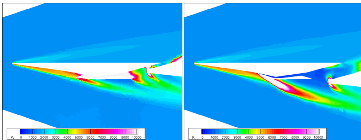
Figure 12: Examples of LEA/Booster interaction with close and open air.
