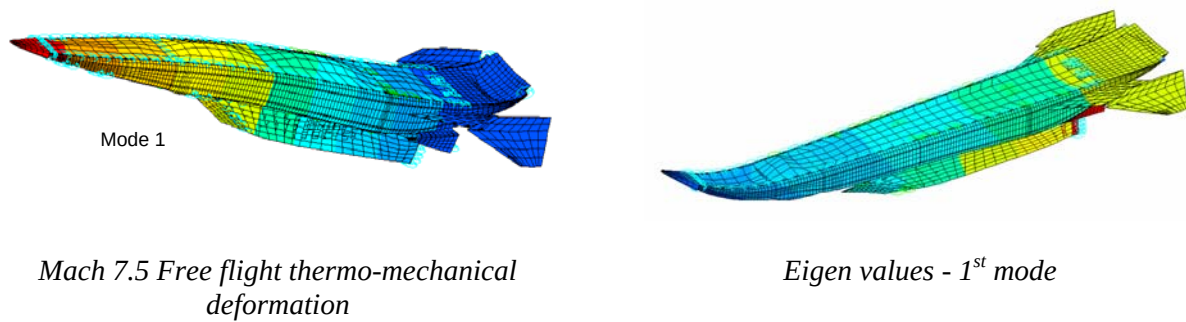
Figure 15: Example of mechanical and thermo-mechanical analysis.
