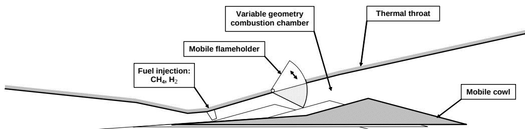
Figure 6: Concept of translating cowl variable geometry engine.
