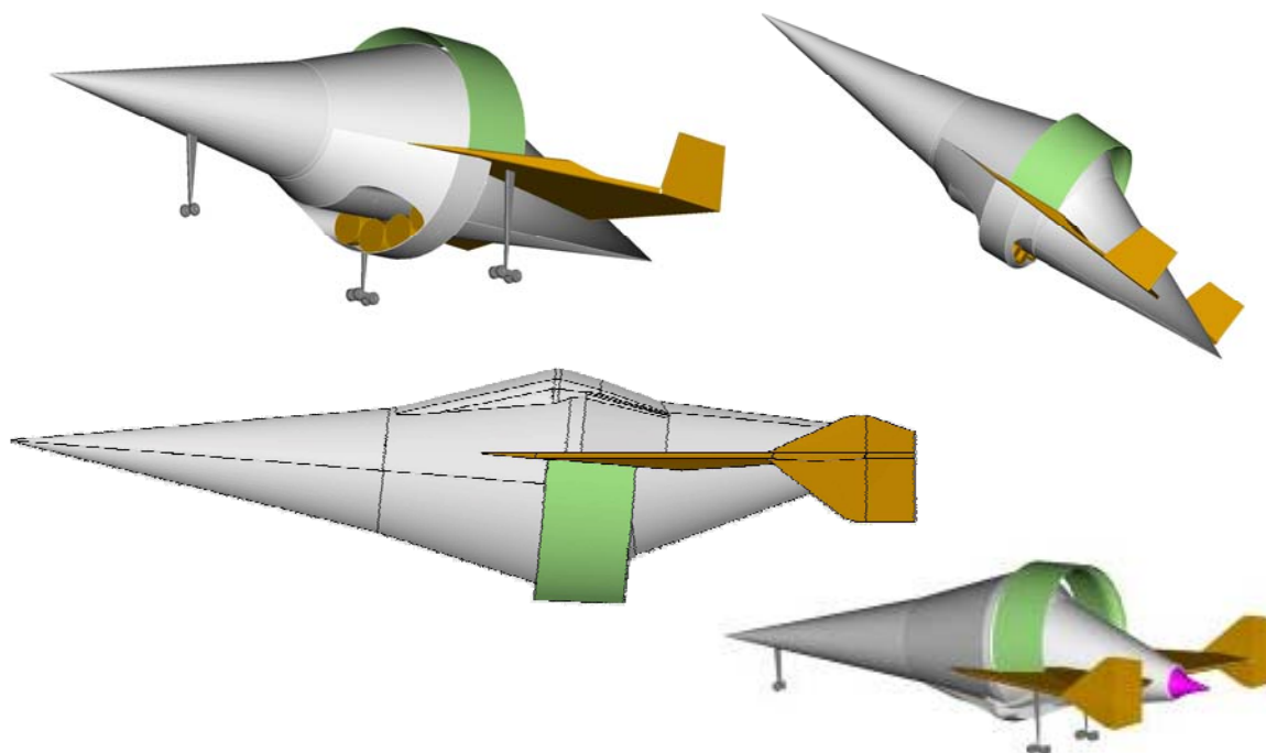
Figure 21: LAPCAT 2 – Mach 8 airplane studied by MBDA.
