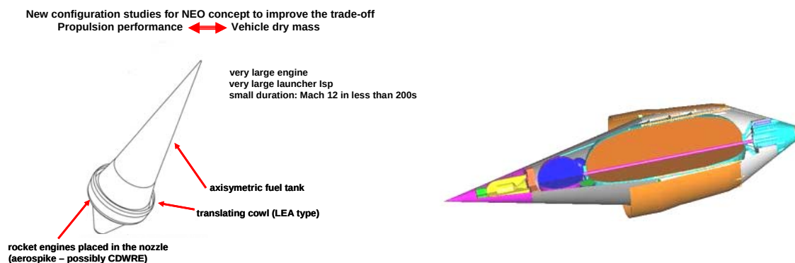
Figure 20: Space launcher NEO concept.
