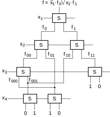
Figure 2.8: Realization of the function in Table 2.1
