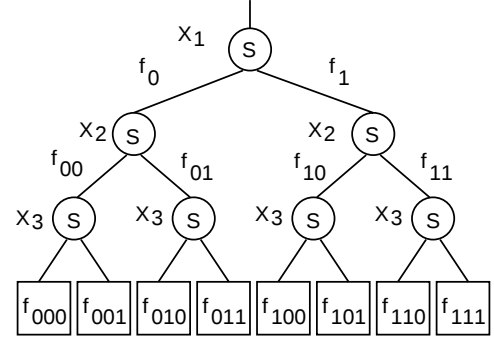
Figure 2.2: Representation of logic functions using the Shannon expansion
