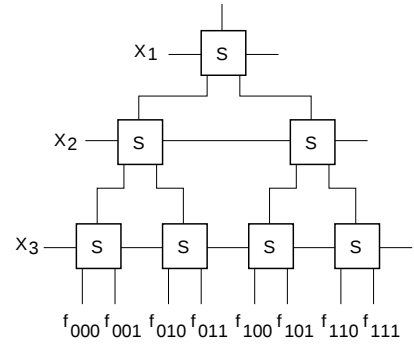
Figure 2.3: Realization of a logic function using multiplexers
