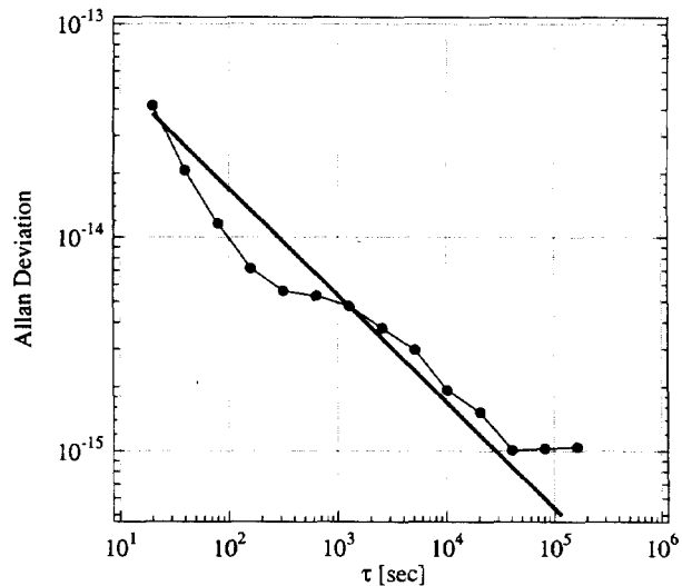
Figure 4. A three-cornered-hat solution for the steered output from the fountain (filled circles). Out to 200 seconds the data is dominated by measurement system noise ( 8 \times 10^{-13}/\tau ). The heavy line represents the white noise level of the fountain at short integration times ( 1.7 \times 10^{-13} \tau^{-1/2} , see Figure 2).
