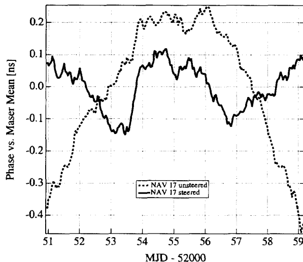
Figure 5. Phase data of both the steered output of the fountain (solid line) and N17 (dashed line) with respect to the USNO maser mean. Both data sets have a least squares fit to a line removed. The parabolic shape of the unsteered data is characteristic of a frequency drift.
