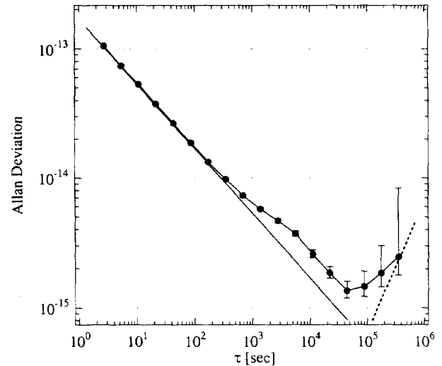
Figure 2. Allan deviation of frequency differences between the fountain and hydrogen maser N17 (filled circles). The stabilities are estimated from a continuous 9 day data set. Also shown are lines representing 1.7 \times 10^{-13} \tau^{-1/2} (solid line), and a drift rate of 8 \times 10^{-16} /day (dashed line).
