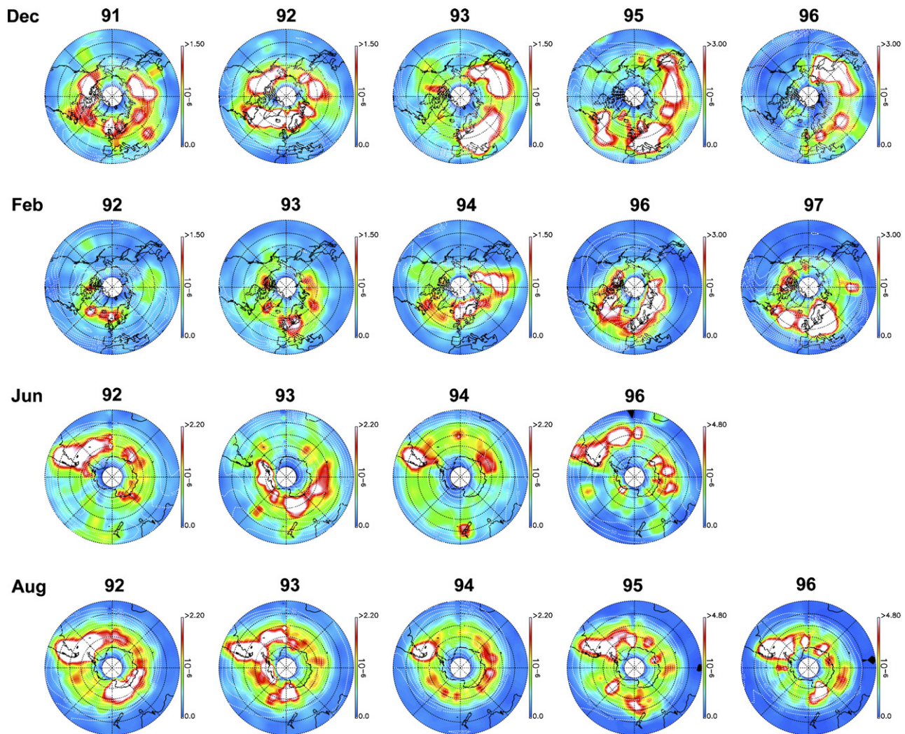
Fig. 4. Multi-year polar maps of 38 km normalized radiance variances during 15–31 December (first-row); 15–28 February (second-row); 15–30 June (third-row); and 15–31 August (fourth-row). Data for northern latitudes are measured from UARS MLS north-looking orbits; data from southern orbits are measured from south-looking orbits. The maps for 1992, 1993, and 1994 (left three columns) are averaged over the half-month period as stated above. The maps for 1995, 1996, and 1997 are averaged over available observation days, which are fewer in number than the half-month period.
