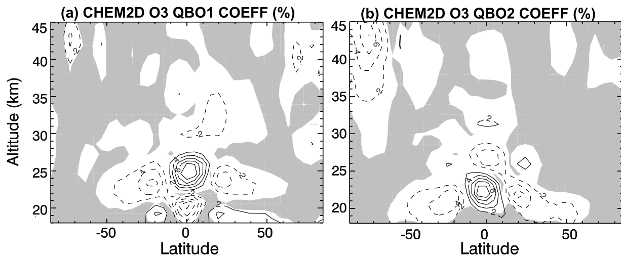
Figure 3. Spatial patterns of the ozone regression coefficients (a) \gamma_{QBO1} and (b) \gamma_{QBO2} , associated with the first and second principal components of the CHEM2D equatorial stratospheric zonal wind, respectively, from the control experiment (EXP0). Coefficients are expressed as the percent change for a one standard deviation change in the principal component time series. Shaded regions are not statistically significant at the 2\sigma level.
