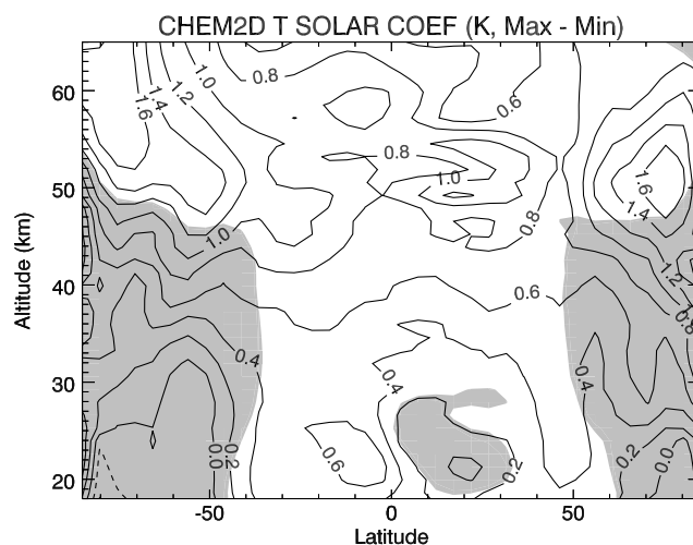
Figure 14. Annual average solar regression coefficients for temperature (change in Kelvin between solar maximum and solar minimum) from experiment 3, which includes varying solar UV, the QBO, and an imposed 11-year variation in planetary wave 1 amplitude. Shaded regions are not statistically significant at the 2\sigma level.
