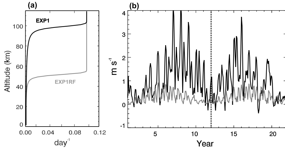
Figure 6. (a) Profiles of the Rayleigh friction timescales in experiment 1 (black curve) and experiment 1RF (gray curve). Experiment 1RF is identical to the profile used by McCormack [2003]. (b) Solar-induced anomalies in the equatorial zonal wind at 50 km from experiment 1 (black curve) and experiment 1RF (gray curve). Dashed vertical line indicates solar maximum.
