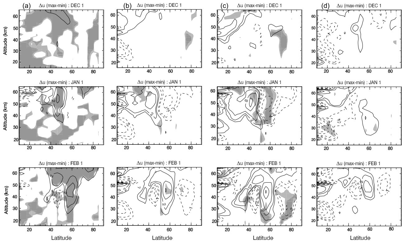
Figure 11. Composite zonal wind differences (in \text{m s}^{-1} , solar maximum minus solar minimum) computed on the first day of December, January, and February from (a) EXP1 with solar cycle and no QBO, (b) EXP2 with solar cycle and QBO, (c) EXP2 for QBO east years only, and (d) EXP2 for QBO west years only. Contours are drawn every \pm 1, \pm 2, \pm 4, \pm 6, \dots . Dashed contours indicate negative values. Light and dark gray shading denotes statistical significance at the 90% and 95% confidence levels, respectively.
