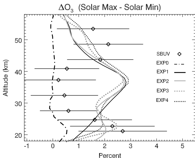
Figure 18. Annual mean solar regression coefficients from model experiments 0–4 averaged between 0° and 20°S, and corresponding solar regression coefficients (diamonds) derived from the 1979–2003 SBUV(2) record with \pm 2\sigma uncertainty estimates [Soukharev and Hood, 2006].
