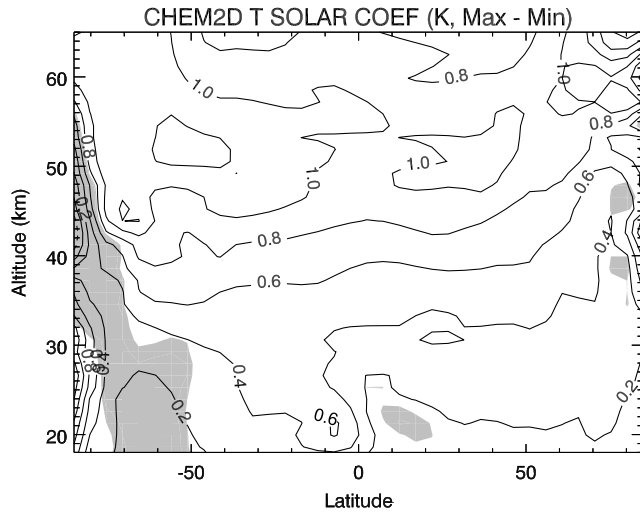
Figure 10. Annual average solar regression coefficients for temperature, expressed as the change (Kelvin) between solar maximum and solar minimum, from experiment 2 that includes both solar UV and QBO effects. Shaded regions are not statistically significant at the 2\sigma level.
