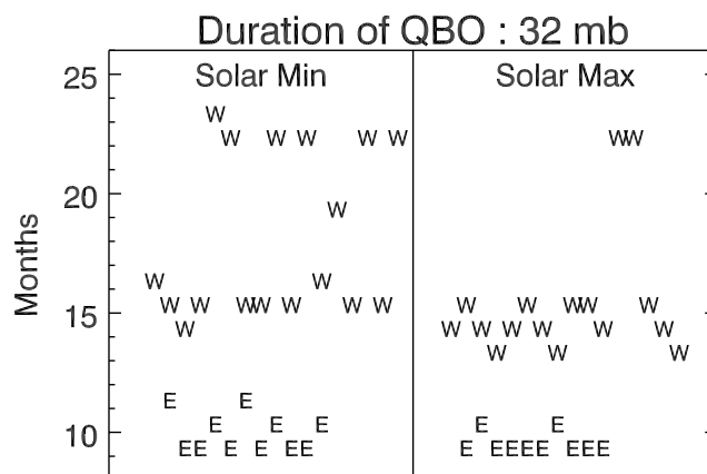
Figure 8. Lengths of individual easterly (E) and westerly (W) model zonal wind QBO phases at 32 hPa, sorted according to the phase of the solar cycle, from experiment 2. The solar irradiance intervals are defined to be within \pm 20 months of the maximum or minimum in UV irradiance.
