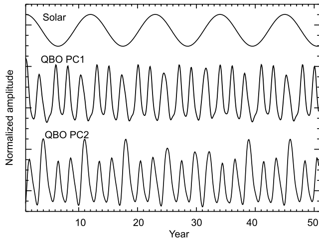
Figure 2. Standardized time series representing solar UV variations and the first two principal components of the zonal wind QBO used in the multiple linear regression model.
