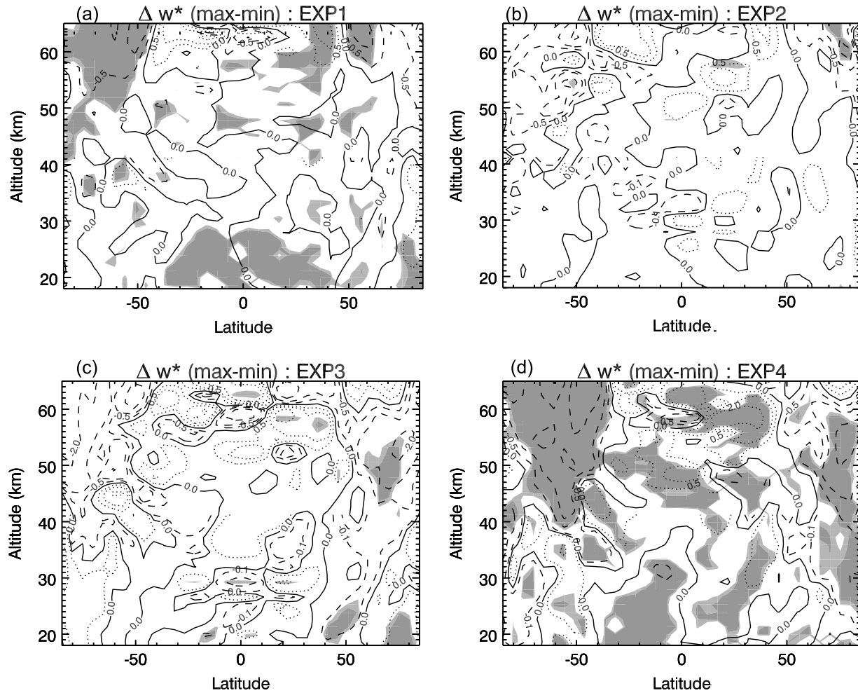
Figure 17. Annual mean composite differences in model vertical velocity \bar{w}^* ( \text{mm s}^{-1} \times 10 ), solar maximum minus solar minimum, from (a) EXP1, (b) EXP2, (c) EXP3, and (d) EXP4. The zero contour is solid, positive contours are dotted, and negative contours are dashed. The \pm 0.1 contours are omitted above 45 km. Light and dark gray shading indicates regions where differences are statistically significant at the 90% and 95% confidence levels, respectively.
