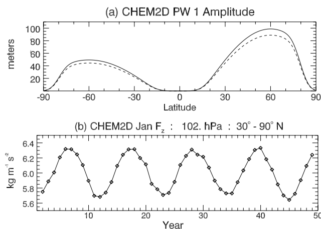
Figure 12. (a) Latitude profile of planetary wave 1 amplitude imposed at the model lower boundary for conditions at solar maximum (dashed line) and solar minimum (solid line) in experiment 3. (b) Time series of the vertical component of the Eliassen-Palm flux at 100 hPa for January, averaged between 30 and 90°N latitude, from experiment 3.
