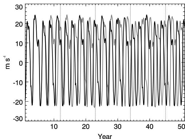
Figure 7. (a) Time series of CHEM2D equatorial zonal winds at 32 hPa from experiment 1 with fixed solar UV (black curve) and experiment 2 with varying solar UV (gray curve). Dashed vertical lines indicate solar maximum.
