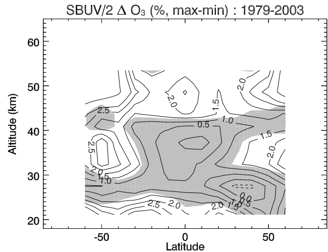
Figure 5. Annual average ozone solar regression coefficients derived from the combined SBUV/(2) ozone profile data set for the period 1979–2003 [Soukharev and Hood, 2006]. Regression coefficients are expressed as the percentage difference between solar maximum and solar minimum. Shaded regions are not statistically significant at the 2\sigma level.
