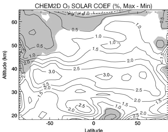
Figure 13. Annual average solar regression coefficients for ozone (percentage change between solar maximum and solar minimum) from experiment 3, which includes varying solar UV, the QBO, and an imposed 11-year variation in planetary wave 1 amplitude. Shaded regions are not statistically significant at the 2\sigma level.
