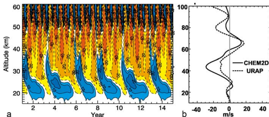
Figure 1. (a) Altitude/time section of CHEM2D equatorial zonal wind from the control experiment (EXP0), solid (dashed) contours denoting westerly (easterly) winds are drawn for 0, \pm 10 , \pm 20 , \pm 40 , and \pm 60 \text{m s}^{-1} . (b) Vertical profiles of annual mean CHEM2D equatorial zonal wind (solid curve) and climatological values obtained from the UARS Reference Atmosphere Project (dashed curve).
