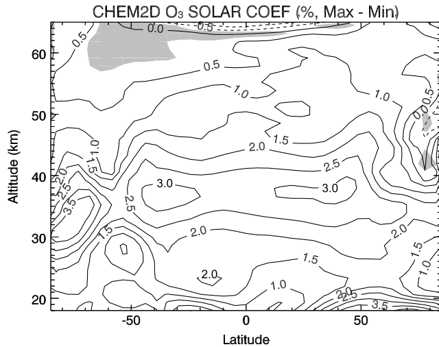
Figure 15. Annual average solar regression coefficients for ozone (percentage change between solar maximum and solar minimum) from experiment 4, which includes varying solar UV and an imposed 11-year variation in planetary wave 1 amplitude. Shaded regions are not statistically significant at the 2\sigma level.
