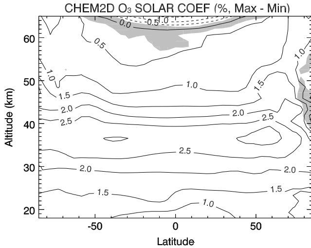
Figure 4. Annual average ozone solar regression coefficients, expressed as the percent change (solar maximum minus solar minimum) from experiment 1, which includes an imposed 11-year cycle in solar UV. Solid contours denote positive values, dashed contours denote negative values, and shaded areas are not significant at the 2\sigma level. Contours are drawn every \pm 0.5\% up to \pm 4\% , and then every \pm 2\% thereafter.
