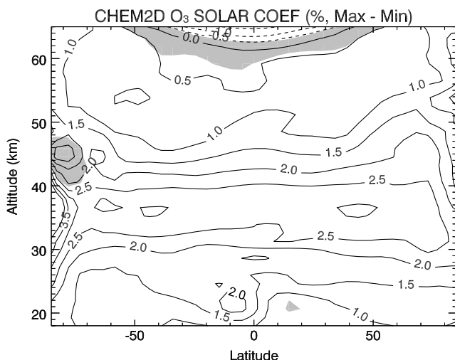
Figure 9. Annual average solar regression coefficients for ozone (percentage change, solar maximum minus solar minimum) from experiment 2, which includes both solar UV and QBO effects. Shaded regions are not statistically significant at the 2\sigma level.
