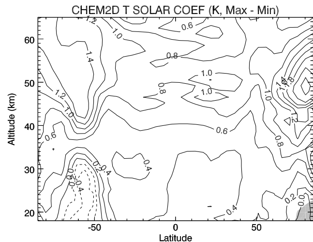
Figure 16. Annual average solar regression coefficients for temperature (change in Kelvin between solar maximum and solar minimum) from experiment 4, which includes varying solar UV and an imposed 11-year variation in planetary wave 1 amplitude. Shaded regions are not statistically significant at the 2\sigma level.
