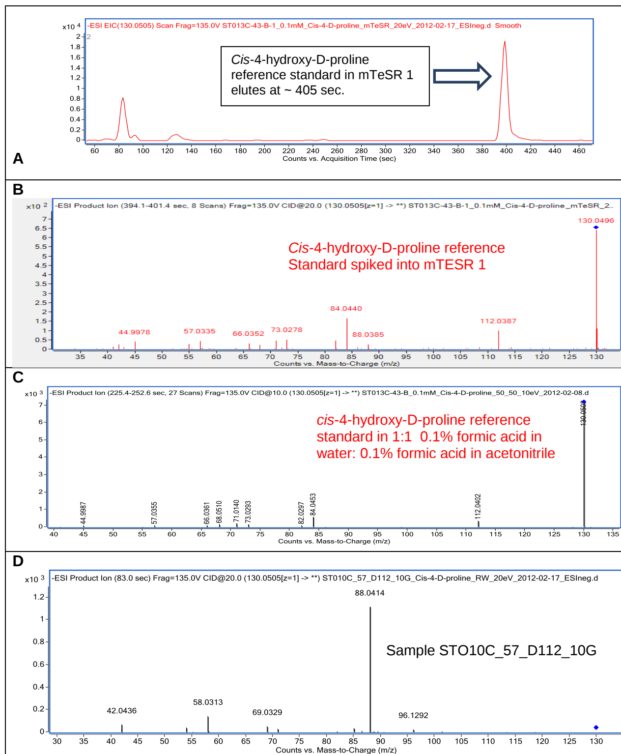
Figure 7. ESI-MS/MS spectra for cis -4-hydroxy-D-proline.
