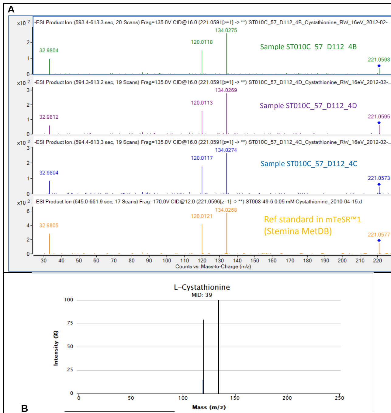
Figure 1. ESI-MS/MS spectra for L-cystathionine.
