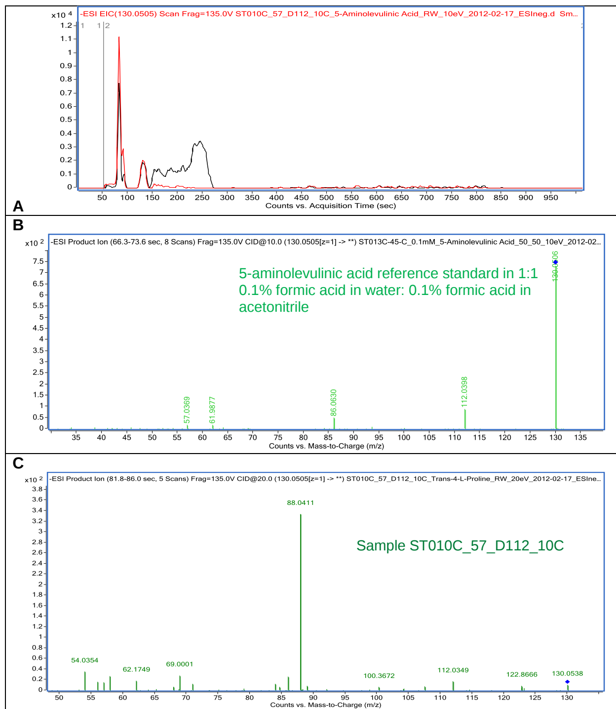
Figure 9. ESI neg EICs and MS-MS spectra for 5-aminolevulinic acid.
