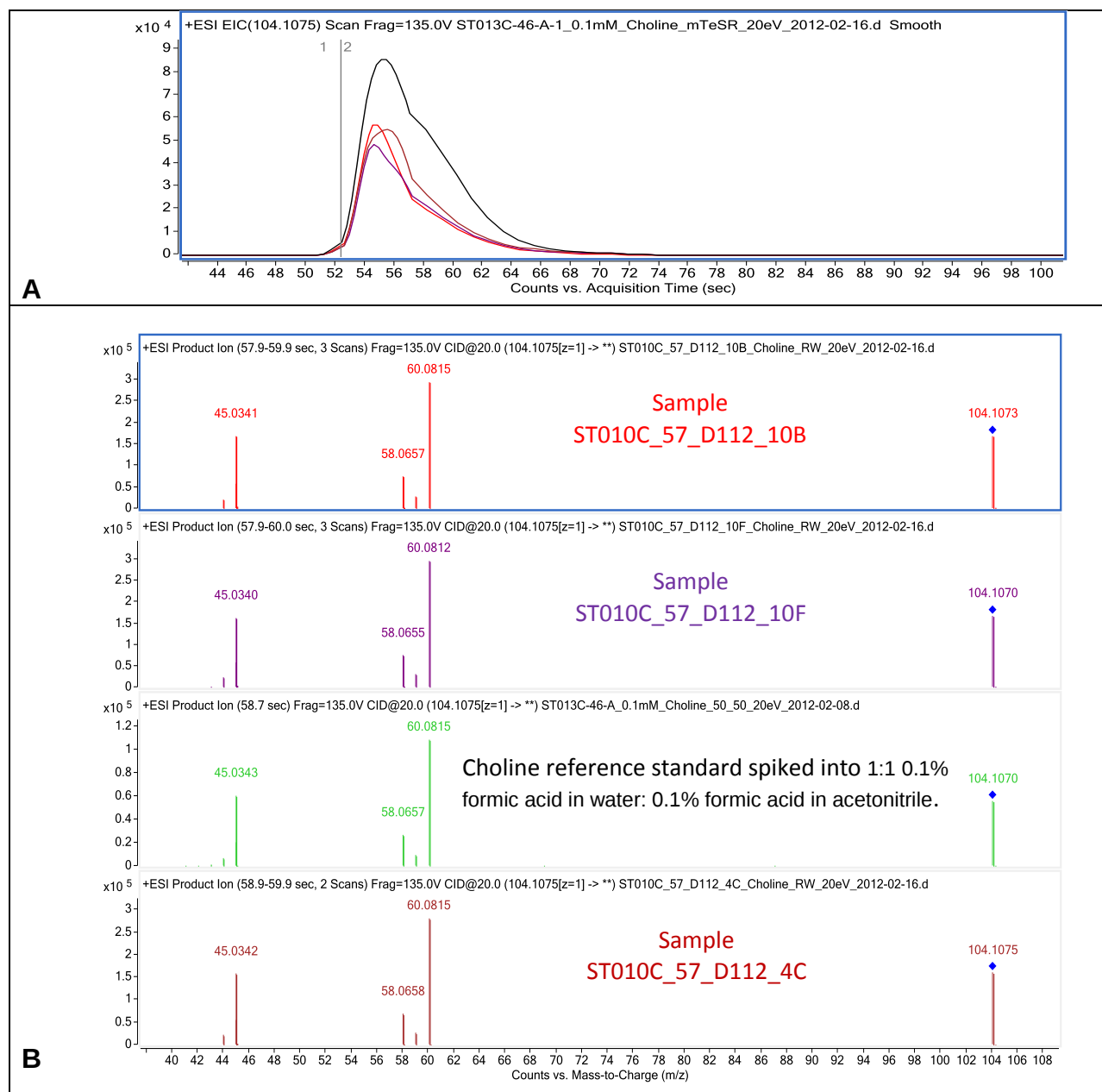
Figure 3. ESIpos MS-MS spectra for choline.
