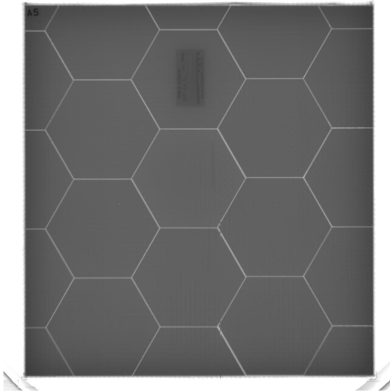
Figure 4 Calibration x-ray Image. Panel A5. Single center high density tile. 150 KVp data. Line pair phantom, Aluminum and carbon rod Image Quality Indicators visible in upper center tile column.
