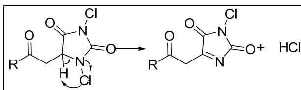
Figure 18. Production of \text{HCl} by chlorinated hydantoin moiety.
