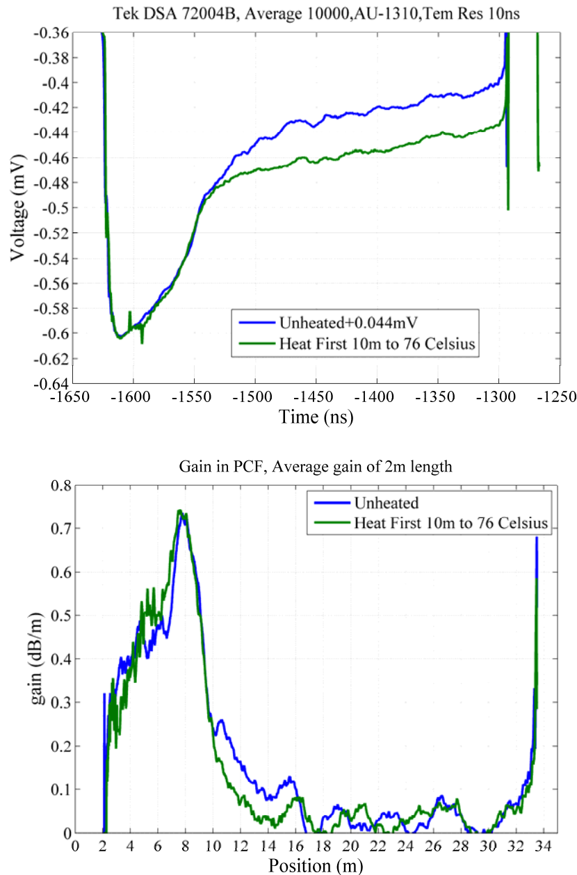
Figure 15. OTDR traces of the AS (top) and calculated gain (bottom) in a \sim 35 m long PGF. Temporal resolution \sim 10 ns. The two curves are for the whole PGF at room temperature (blue) and for the first 10 m heated to 76^\circ\text{C} (green).
