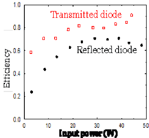
Fig. 2. Combination efficiency for reflected diode (circular spots) and transmitted diode (square spots) vs. input power.
