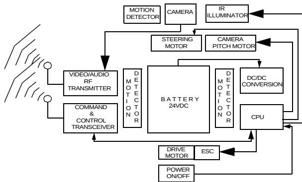
Figure 6 : Overall electronic systems architecture (signal-bus only)
