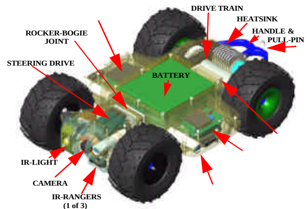
Figure 5 : See-thru packaging design for DR vehicle
