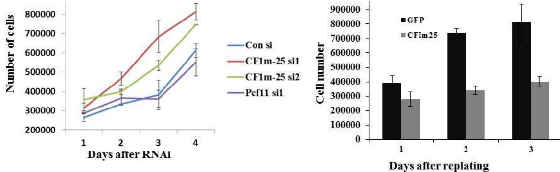
Figure 7. Left panel. Graph shows effect of different siRNA's on cell growth. Right panel. Graphical representation of the effect of CFIm25 overexpression on cell growth.
