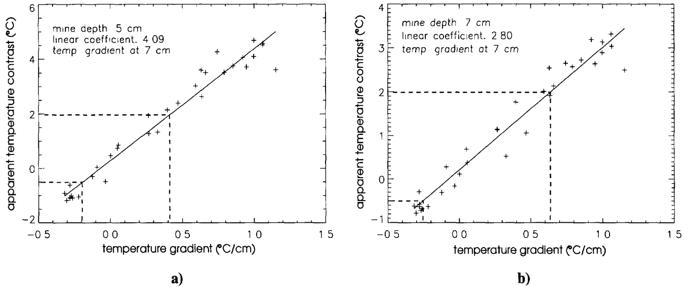
Figure 3: These two plots are derived from figure 2b. The + symbols show the apparent temperature contrasts corresponding to the temperature gradients. The straight lines are obtained from a standard first order polynomial fits through these points.
