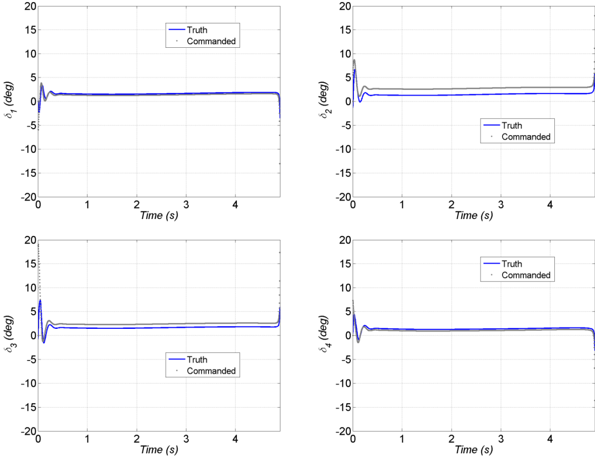
Figure 31. Nonlinear system simulation – individual canard deflection commands.
