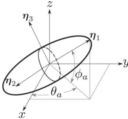
FIG. 10. Definition of ellipsoid's orientation with respect to the largest semiaxis.
