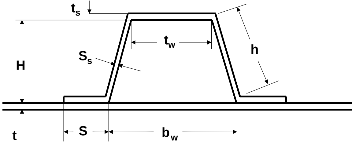
Figure 5. Hat-Stiffener Dimensions
