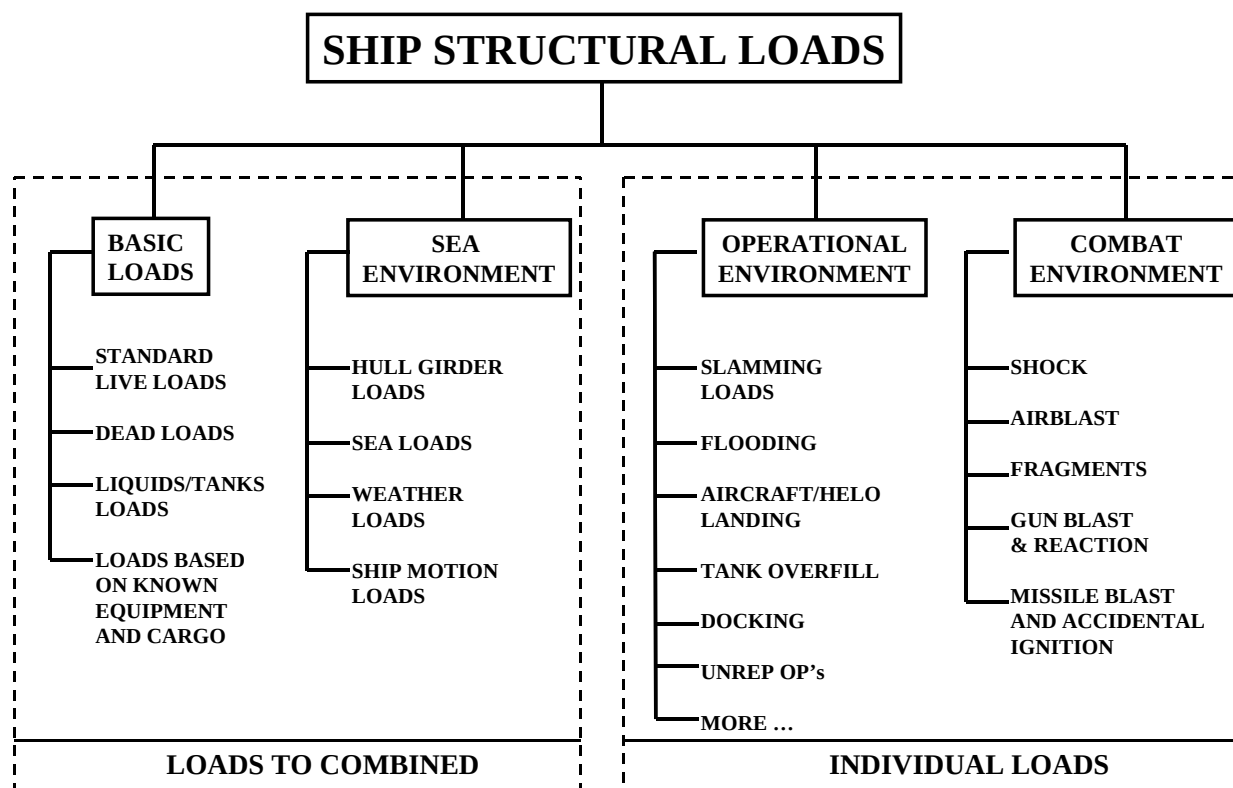
Figure 1. Categories of Ship Structural Loads
