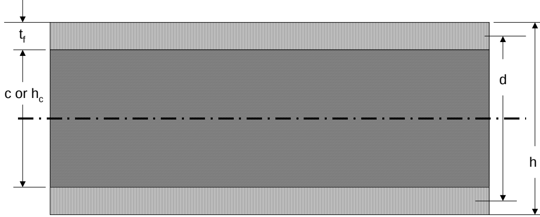
Figure 3. Sandwich Panel Dimensions
