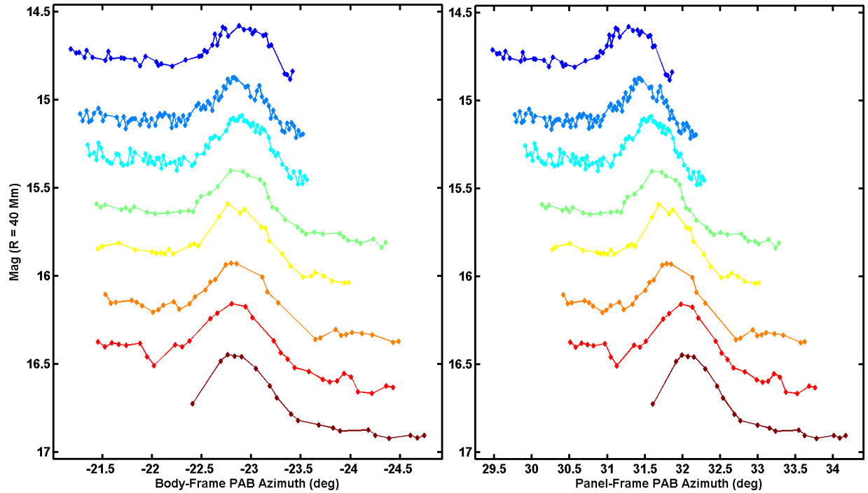
Figure 6. The eight-glnt Galaxy 15 sequence detected during 2010 Nov 14 to Nov 27 (as color coded in Figure 3), plotted as a function of body-frame phase-angle bisector azimuth (left) and solar-panel-frame phase-angle bisector azimuth (right), with 0.25 magnitude vertical separations added between the successive nights. The fact that the peaks align in terms of the body-frame PAB angle on the left (and not in terms of the panel-frame PAB angle on the right) strongly suggests that this glint originates from a body-mounted component on the satellite (and not a panel-mounted component).
