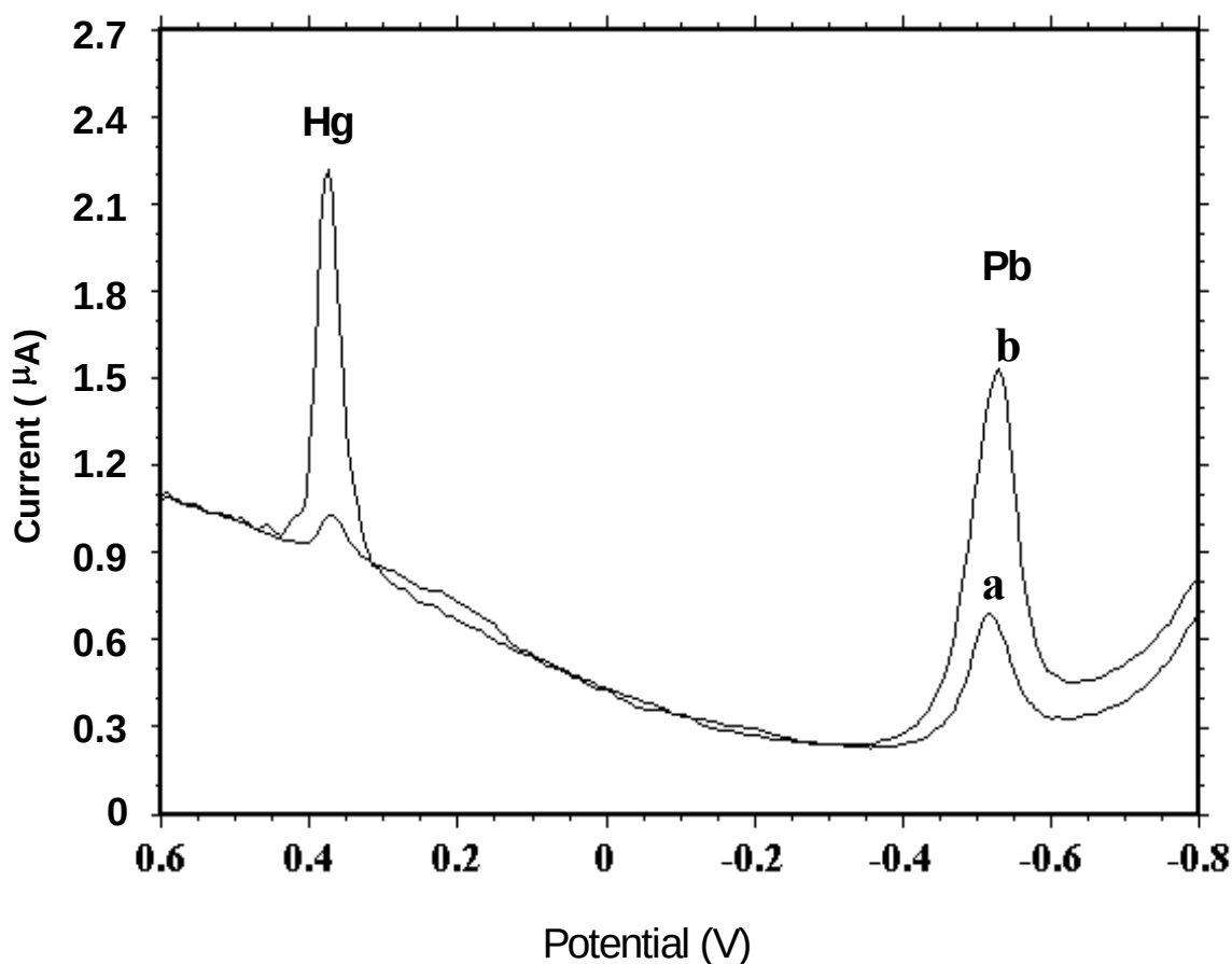
Figure 7: Voltammetric response after (a) 2 minute preconcentration in 30 ppb. Pb 2+ /160 ppb. Hg 2+ , and (b) 20 minute preconcentration in 1.5 ppb. Pb 2+ /3 ppb. Hg 2+
