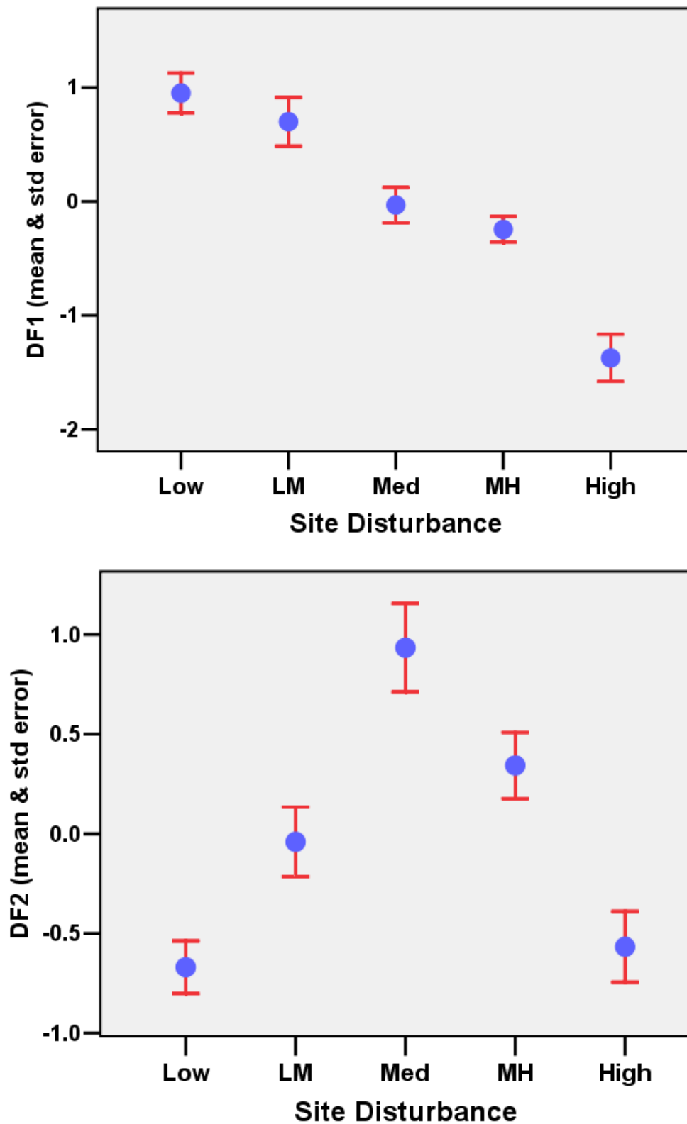
Figures 48 (upper) and 49 (lower). Floristics Ground Cover Guild Discriminant Functions DF1 and DF2. The values are mean and standard error.
