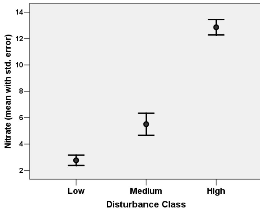
Figure 23. Soil Mineralization Potential experiment. Ammonium ( \text{NH}_4^+ ) (above) and nitrate ( \text{NO}_3^- ) (below) soil concentrations after laboratory incubation for four days. Concentrations are N-mg/kg.
