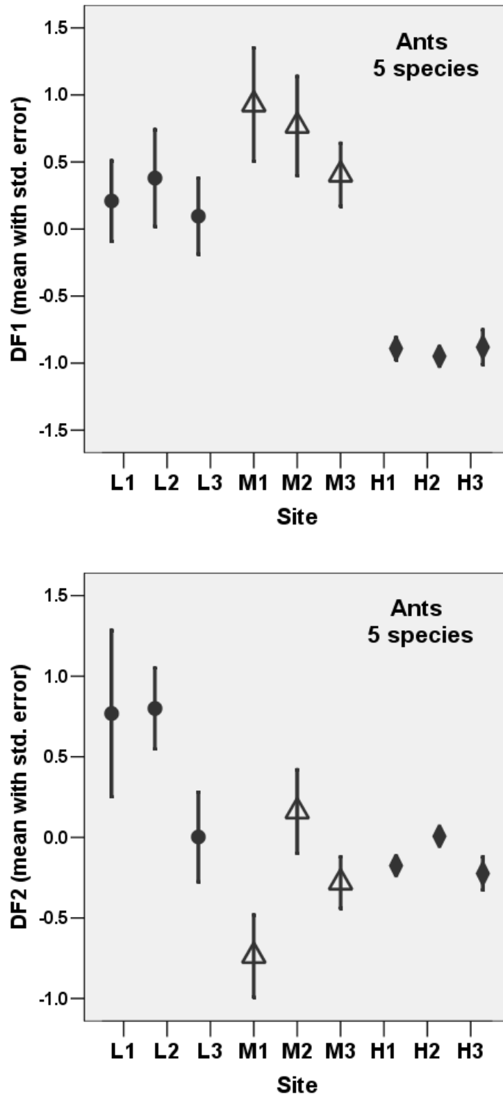
Figure 28. Ground/litter Ant community (5 species, Dorymyrmex smithi deleted) Discriminant Analysis scores, discriminant function 1 (above) and discriminant function 2 (below). Bonham Creek and Sally Branch (9 sites, 2000-2001-2002). Total number of ants = 554, 0.54% of original 28 species.
