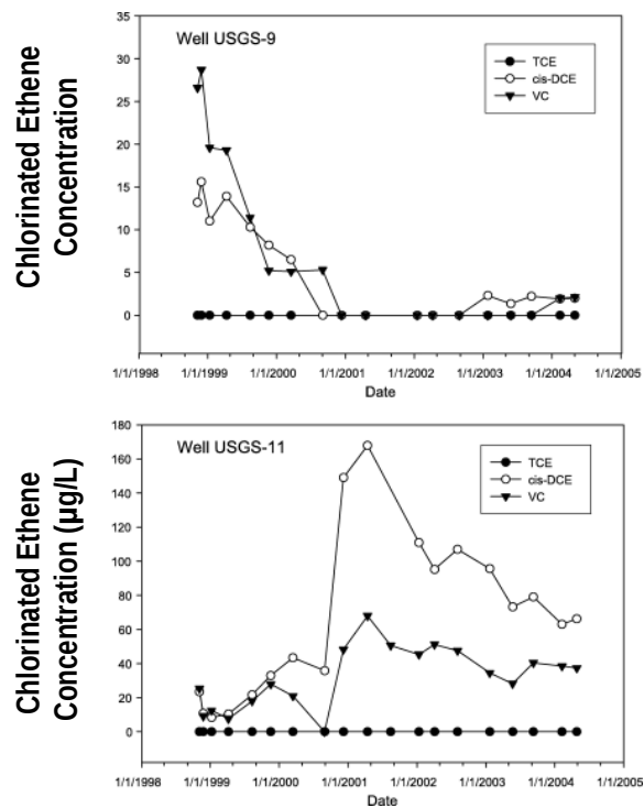
Figure A-3. Concentration Changes 75 m Downgradient of the Treated Source Area Between 1998 and 2004 (Chapelle et al., 2005)
