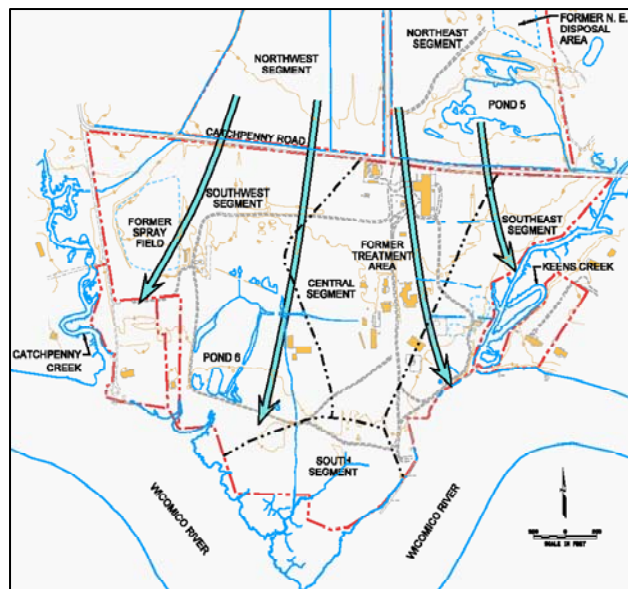
Figure B-2. Groundwater Flow at Creosote Site (RITS 2006: DNAPL Management Challenges)
