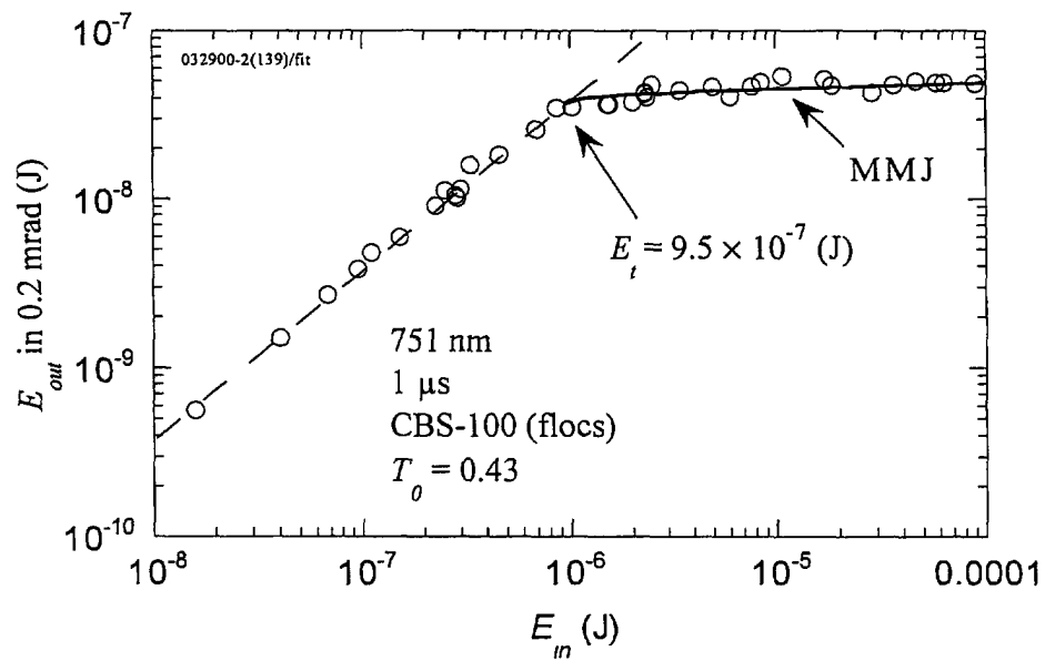
Figure 15. Threshold determination in a sample of CBS-100 (flocs) for long pulses: MMJ fit
