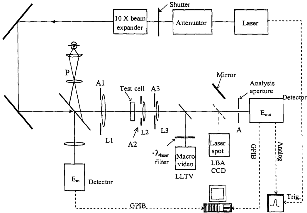
Figure 1. Measurement system LLTV is a low level TV which allows the observation of particles' movement in the cell illuminated by the projector P, but the light is off during the nonlinear transmission measurements. LBA is a laser beam analyzer with a CCD camera which allows the observation of the laser spot when the angled mirror is in position. The output pulse can be seen on an oscilloscope and the data are collected by a dedicated computer.
