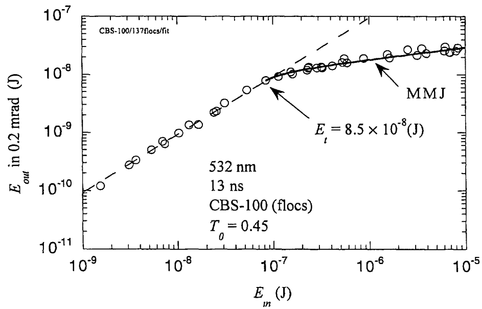
Figure 11. Threshold determination in a sample of CBS-100 (flocs) for short pulses: MMJ fit
