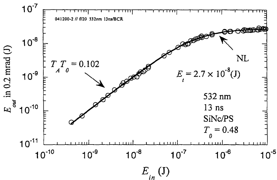
Figure 5. Curve fit for SiNc in polystyrene
