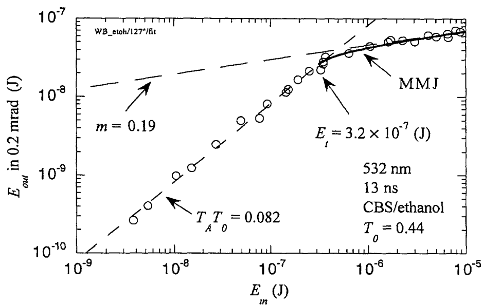
Figure 4. Curve fit for CBS in ethanol
