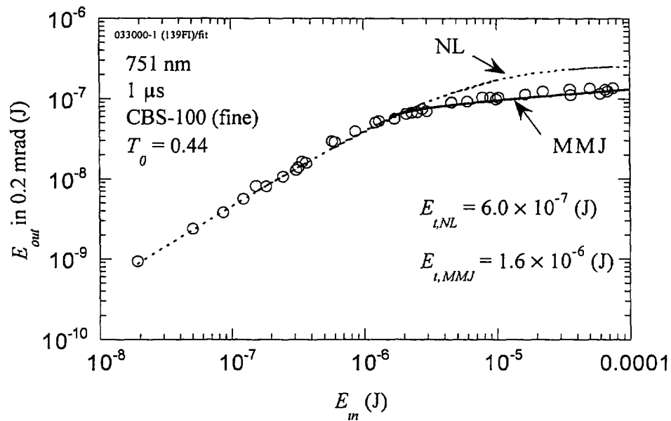
Figure 13. Threshold determination in a sample of CBS-100 (fine) for long pulses. MMJ and NL fits
