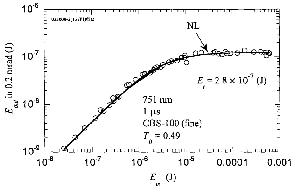
Figure 14. Threshold determination in a sample of CBS-100 (fine) for long pulses: NL fit
