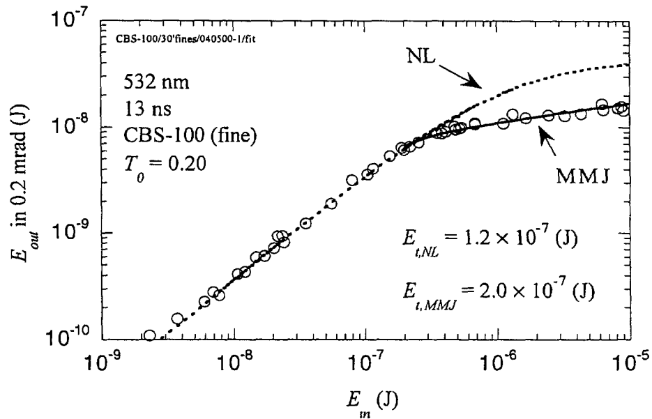
Figure 9. Threshold determination in a sample of CBS-100 (fine) for short pulses: MMJ and NL fits
