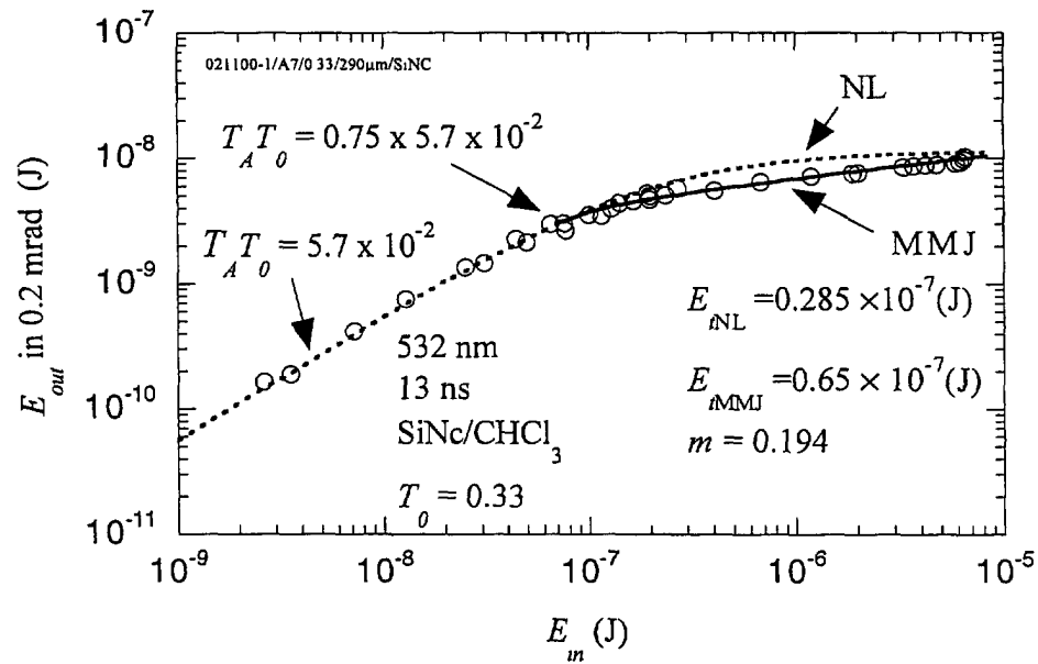
Figure 6. Curve fit for SiNc in chloroform
