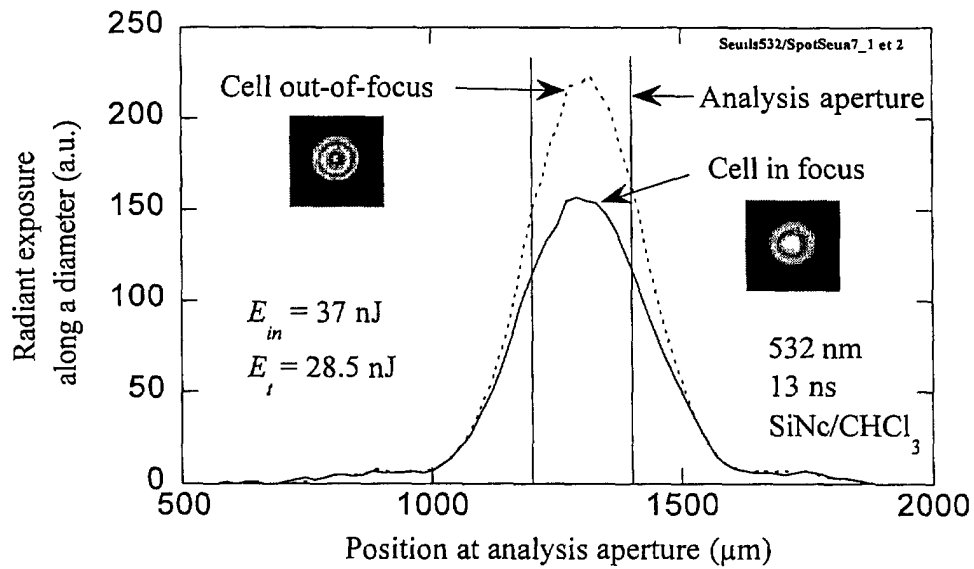
Figure 7. Laser spots in the analysis plane when the focus of L1 is in the cell and out of the cell. The figure shows that the change in measured energy is much larger through the aperture than in the full spot.
