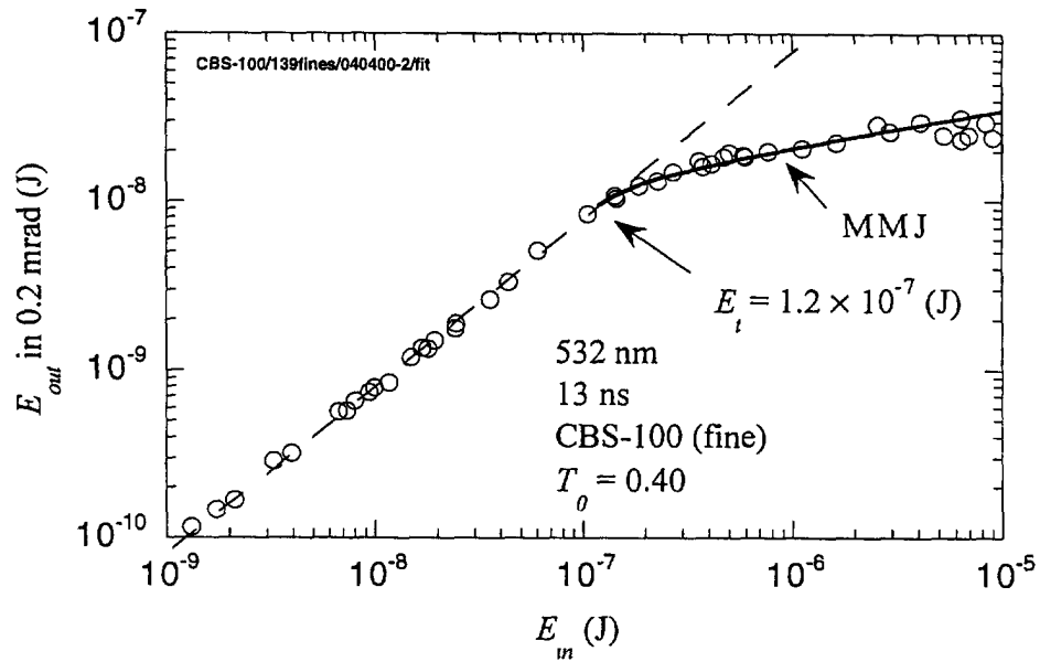
Figure 8. Threshold determination in a sample of CBS-100 (fine) for short pulses: MMJ fit
