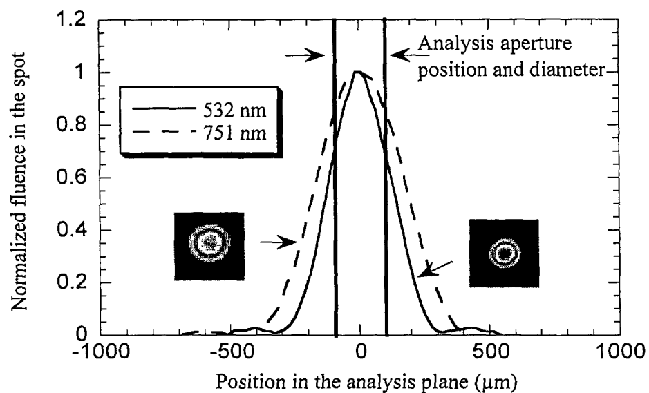
Figure 2. Spot profiles and aperture position in the analysis plane, the photographs show that the constant fluence contours in the spot are circular.
