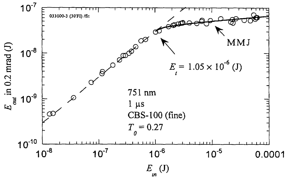
Figure 12. Threshold determination in a sample of CBS-100 (fine) for long pulses. MMJ fit
