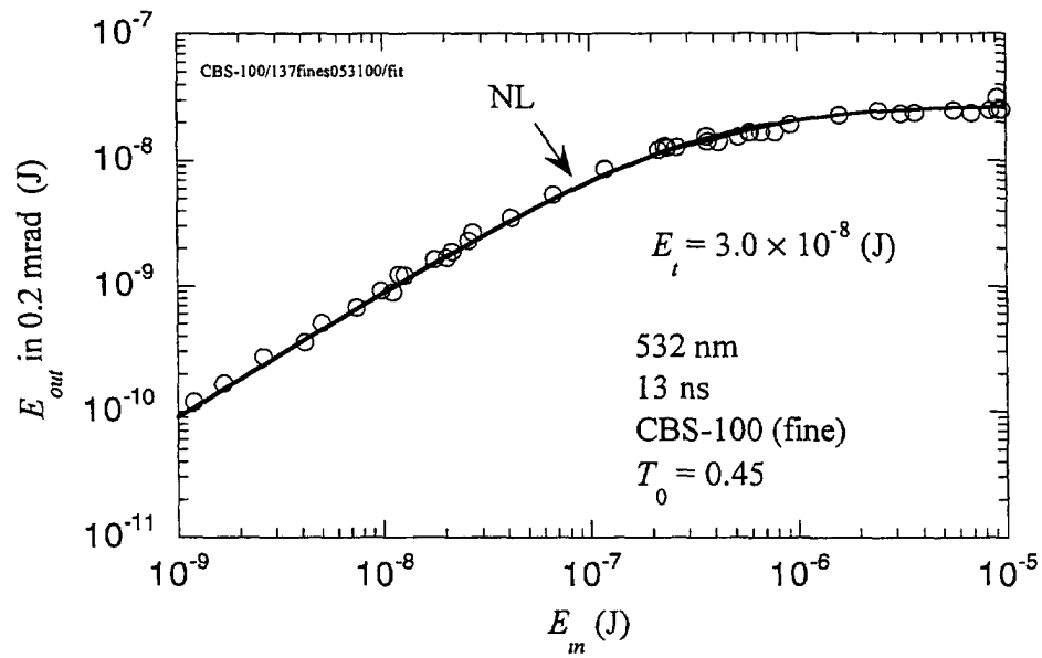
Figure 10. Threshold determination in a sample of CBS-100 (fine) for short pulses: NL fit
