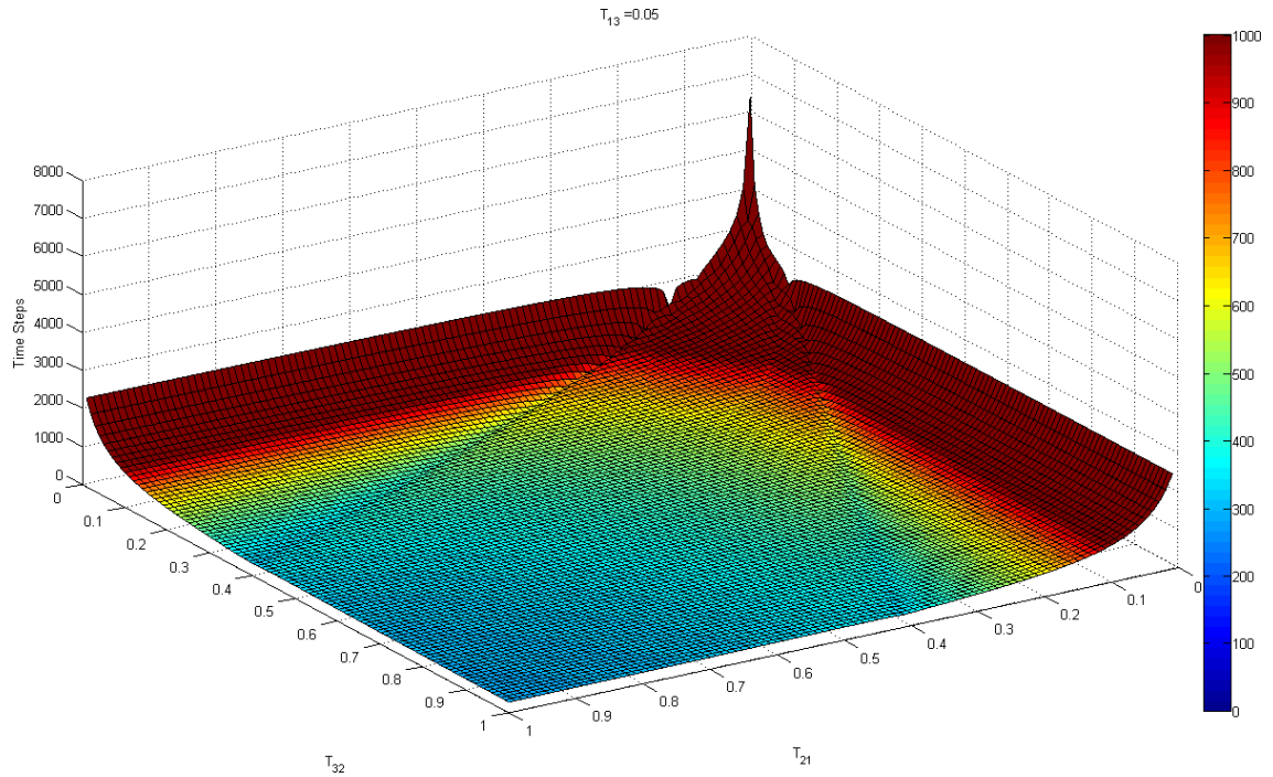
Figure 6.4. Value (a) and Time Step (b) Convergence Results for T_{13} = 0.05 , 0.01 \leq T_{21} \leq 1 , and 0.01 \leq T_{32} \leq 1 . (This figure is presented in color; the black and white reproduction may not be an accurate representation.)
