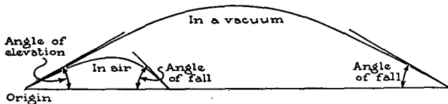
(Note the tremendous decrease in range caused by air resistance.) FIGURE 2.—Comparison of a trajectory in a vacuum and one in air.
