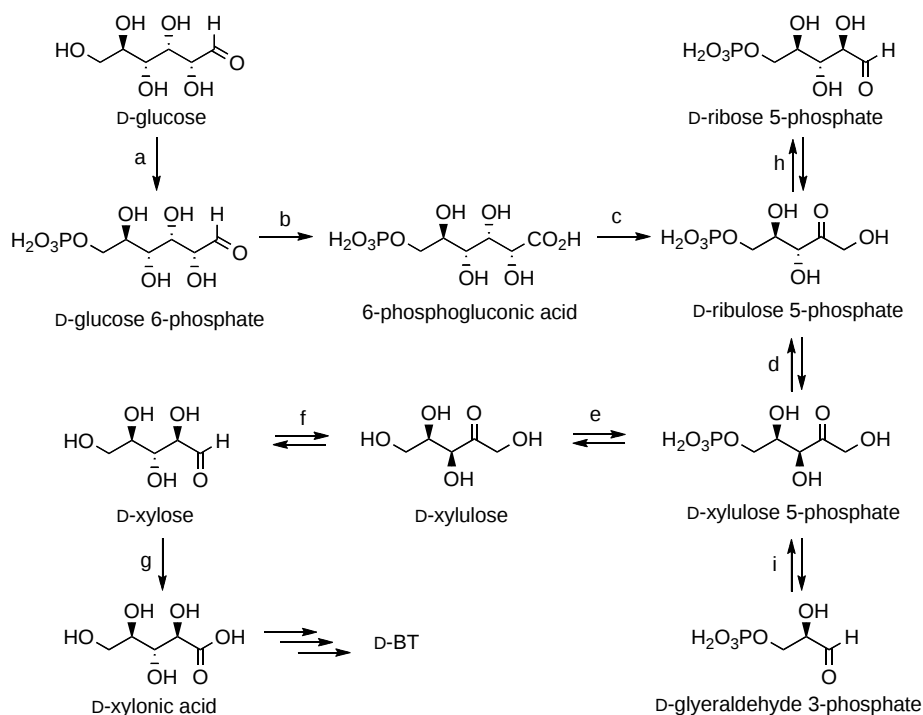
Figure 1. Microbial Synthesis of D-Xylonic Acid from D-Glucose. (a) carbohydrate phosphotransferase ( ptsG , crr ); (b) D-glucose 6-phosphate dehydrogenase ( zwf ); (c) 6-phosphogluconate dehydrogenase ( gnd ); (d) D-ribulose phosphate epimerase ( rpe ); (e) phosphatase; (f) D-xylulose isomerase ( xylA ); (g) C. crescentus D-xylose dehydrogenase ( xdh ); (h) D-ribose 5-phosphate isomerase ( rpiA , rpiB ); (i) transketolase ( tktA , tktB ).
