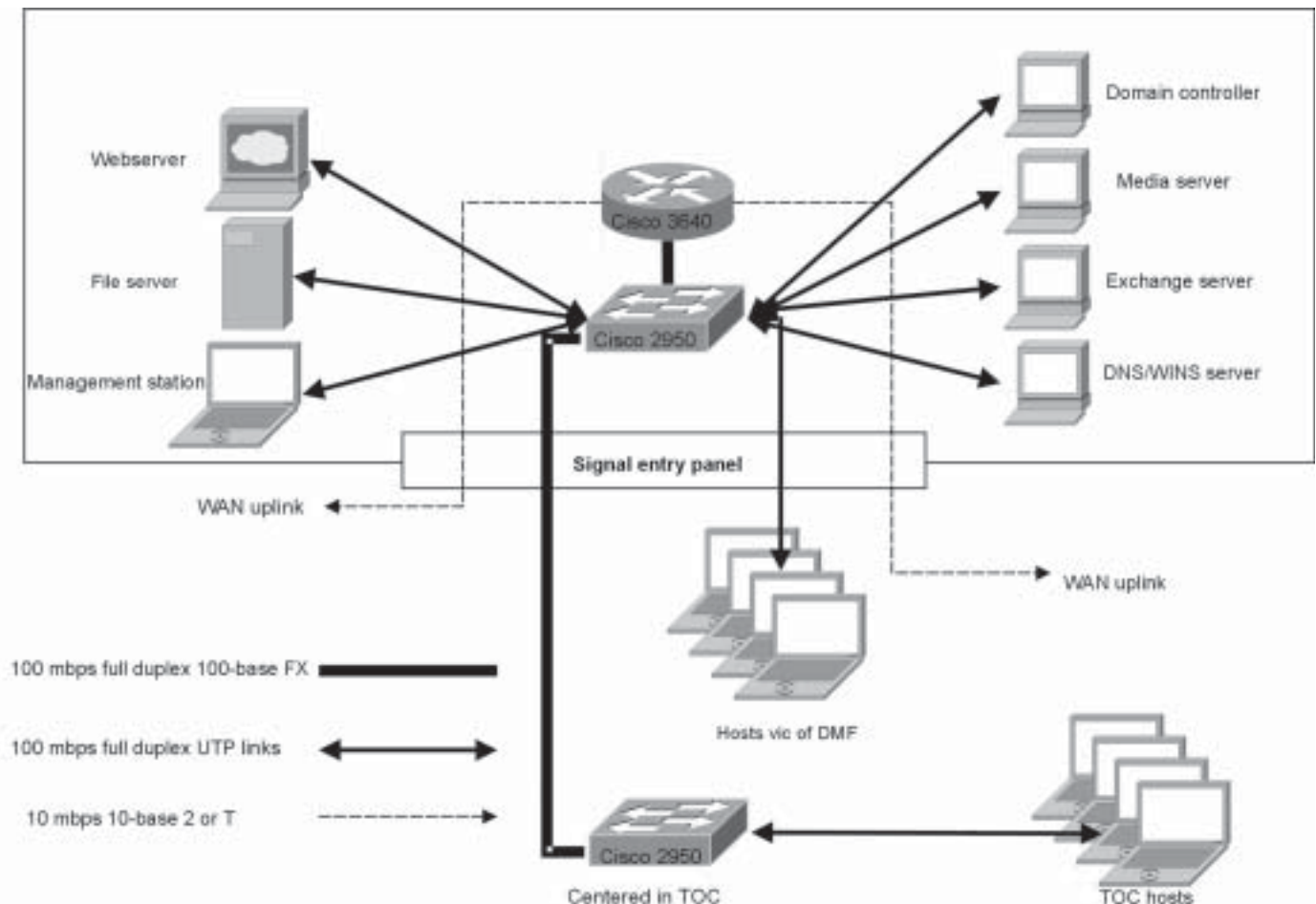
Figure 24. 10th Mountain Division's TOC infrastructure. The boxed area at the illustration's top shows the setup inside the data-management facility truck, mounted on 19-inch racks.
