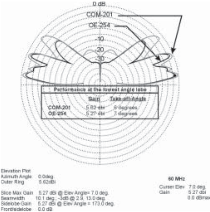
Figure 35. Comparison of COM-201 to OE-254 at 60 mhz.
