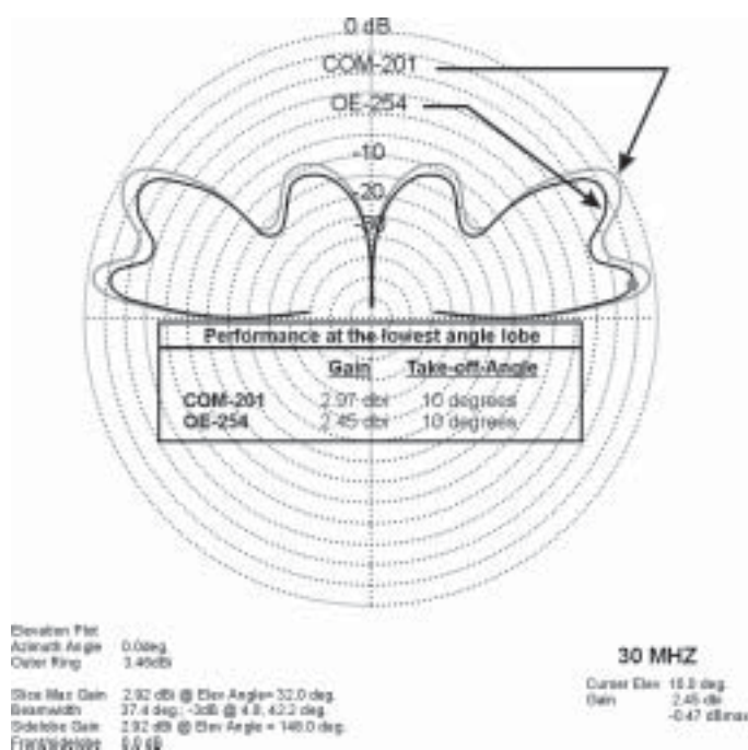
Figure 33. Comparison of COM-201 to OE-254 at 30 mhz.
