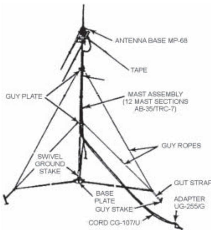
Figure 31. The RC-292 is a general-purpose, stationary, ground-plane antenna used to increase the transmission/reception range of tactical frequency-modulation radio sets. The radiating and ground-plane elements must be adjusted to the proper length for a particular operating frequency. The RC-292's technical characteristics are: frequency range, 20-76 mhz; planning range, about twice the planning range of a radio set using a quarter-wave whip antenna; height when erected, 11.28 to 12.56 meters (37 to 41.2 feet); and weight, about 19.5 kilograms (43 pounds).
