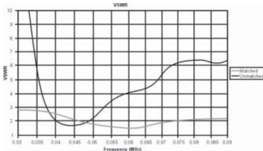
Figure 39. Comparison of tuned COM-201 vs. untuned antenna.
