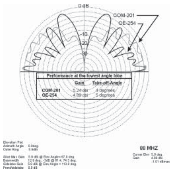
Figure 37. Comparison of COM-201 to OE-254 at 88 mhz.
