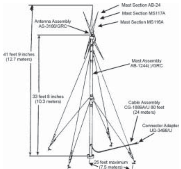
Figure 32. The OE-254 is a general-purpose, stationary, broadband, omni-directional antenna used to extend the range of tactical FM radio sets. Under normal field conditions, the antenna will be mast-mounted. Once installed, the OE-254 doesn't have to be taken down for adjustment when a new frequency band is assigned to the radio net. The OE-254's technical characteristics are: frequency range, 30-88 mhz; planning range, 57.9 kilometers (36 miles), average terrain, or 48.3 kilometers (30 miles), difficult terrain; radio-frequency power capability, 35 watts nominal; antenna-erection time (one person), 15 minutes; height when erected, 12.8 meters (42 feet); input impedance to radio, 50 ohms; and weight, 20.4 kilograms (45 pounds).
