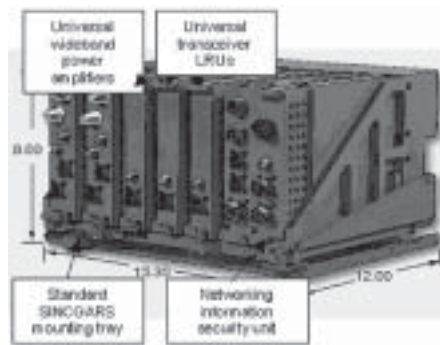
Figure 24. Boeing's design of the vehicular JTRS Cluster 1 radio.
