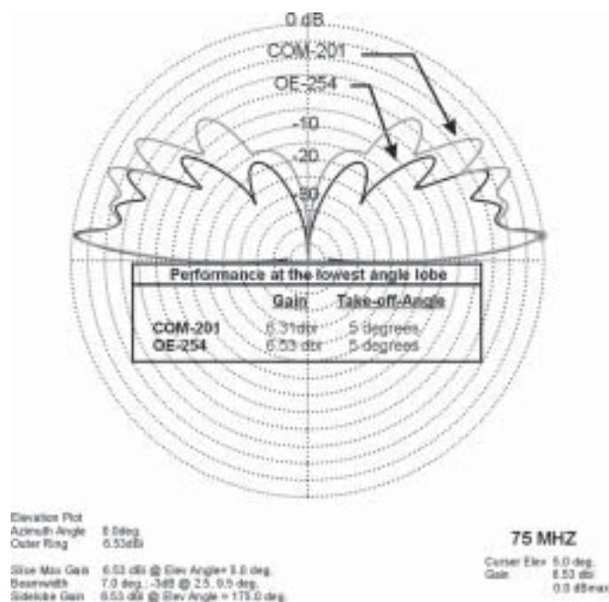
Figure 36. Comparison of COM-201 to OE-254 at 75 mhz.
