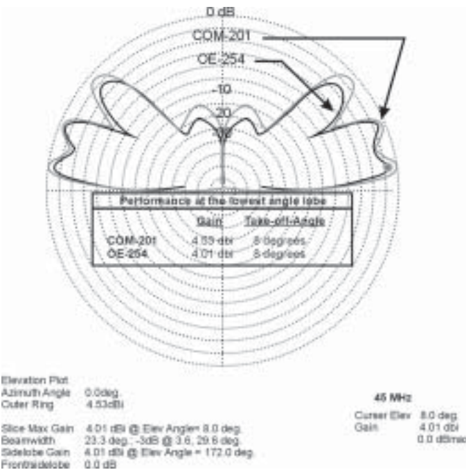
Figure 34. Comparison of COM-201 to OE-254 at 45 mhz.
