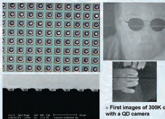
Figure 81. Focal Plane Arrays – Indium Bumps and Hybridization to ROIC. Source: Author.
