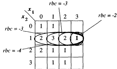
Figure 7. Selection of the First Implicant Using the Dueck and Miller Heuristic in the One-Pass Method.
