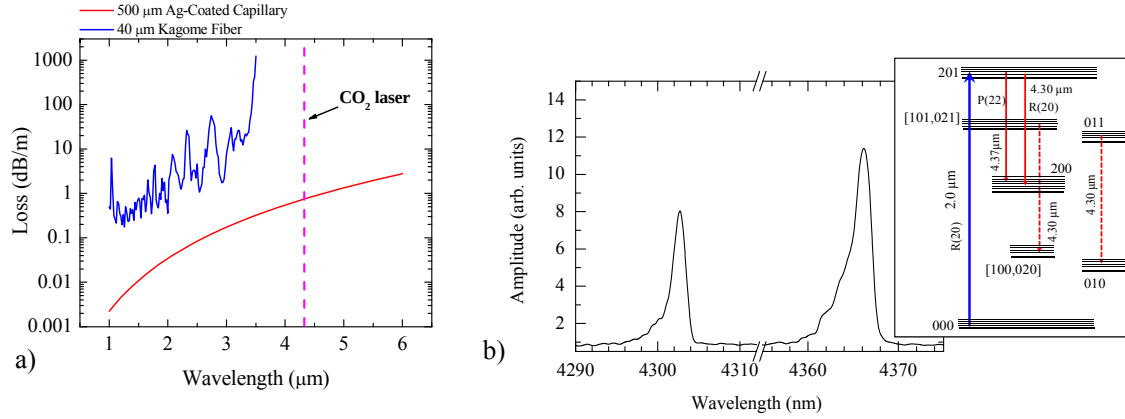
Fig. 3 a) Transmission of a 500 μm diameter silver coated hollow waveguide along with transmission of a traditional kagome silica HCF in the mid-IR region, and b) optically pumped CO 2 capillary laser showing emission in the 4.3 μm region. Inset shows the pump and lasing transitions in a vibrational energy level diagram of CO 2 .
