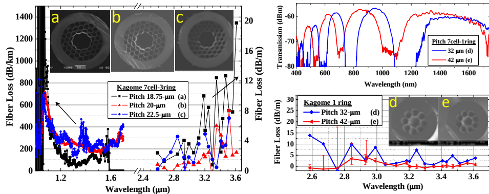
Fig. 7 (a-c): Kagome HCF having hypocycloid core with 3 cladding rings and 7 cell defects with pitches of 18.75 \mu\text{m} , 20 \mu\text{m} , and 22.5 \mu\text{m} and core diameters of 85-93.75, 87.5 – 92.5, and 85-93.75 \mu\text{m} ; (d-e): kagome fibers with hypocycloid core structure having 1 cladding ring with pitches of 32 \mu\text{m} and 42 \mu\text{m} and core sizes of 58 \mu\text{m} and 64 \mu\text{m} respectively. (left) fiber loss versus wavelength in the near and mid-IR for 3 ring hypocycloid fibers (a)-(c). (Right top) Transmission of 1 ring kagome hypocycloid core fibers in the near-IR. For reference, the loss in the 42 \mu\text{m} pitch fiber (red) is measured to be 5 dB/m at 1.50 \mu\text{m} wavelength. (Right bottom) mid-IR loss of 1 ring kagome hypocycloid core fibers measured with the OPA. Error bars are generated from repeatability of two cut-backs of fiber length 0.8 and 2.0 m.
