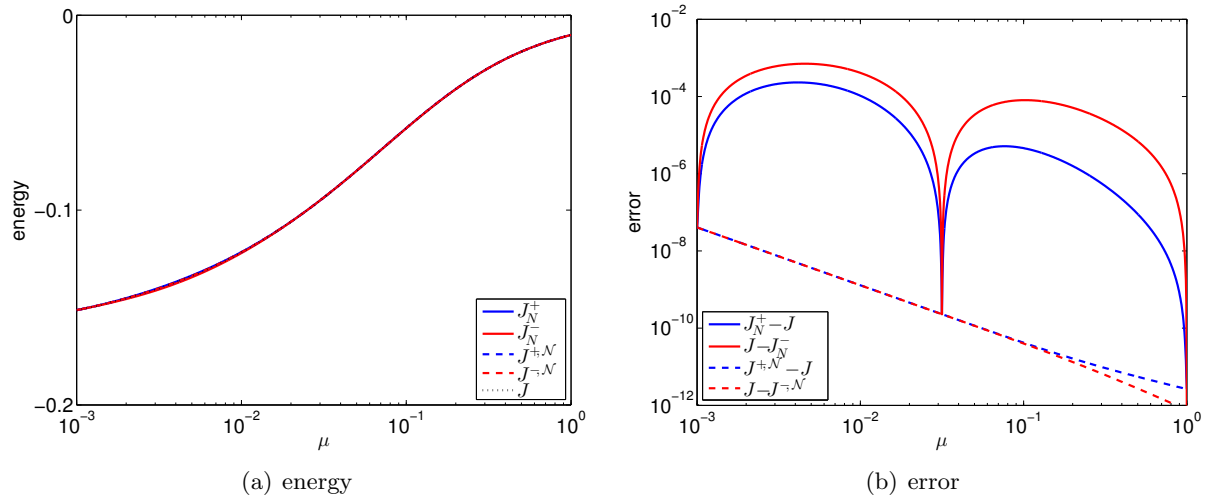
Figure 1: The behavior of the bounds for the reaction-diffusion problem for n_e = 128 and N = 3 . ( J : truth; J_N^\pm : reduced basis bounds; J^{\pm, \mathcal{N}} : finite element bounds)
