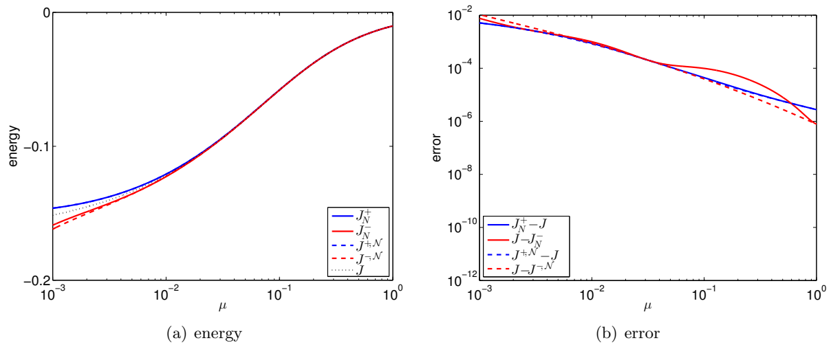
Figure 2: The behavior of the bounds for the reaction-diffusion problem for n_e = 4 and N = 3 . ( J : truth; J_N^\pm : reduced basis bounds; J^{\pm, \mathcal{N}} : finite element bounds)
