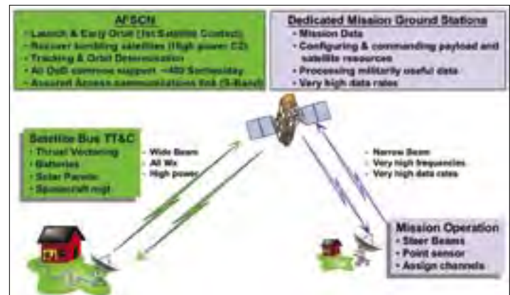
Figure 2. Satellite Control.
