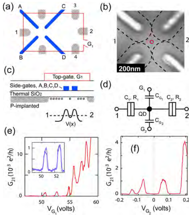
FIG. 1. (Color online) Schematics show (a) the top and (c) the cross sectional views of our silicon single-electron transistor structure. In (a) the solid thick line, the shaded regions, and the rectangular area depict the side gates, phosphorous-implanted Ohmic leads, and the boundary of the top gate, respectively. The schematic potential profile along the 1-2 direction under single electron tunneling condition is shown as the inset (lower right) in (c). (b) Scanning electron micrograph of 70-nm-wide side gates defined by electron-beam lithography, taken before the top gate is defined. The gap between neighboring side gates is \sim 160 nm. The dashed lines illustrate the depletion region under single-electron transistor operating condition. The 20 nm diameter circle depicts the location of the quantum dot as discussed in the text. (d) The SET equivalent circuit used in the analysis for capacitances. (e) Transfer characteristics vs the top-gate voltage at V_A = V_B = V_C = V_D = 0 V and V_{21} = 8 mV. The inset shows the up and down traces. (f) Transfer characteristics controlled by the side-gate voltage at V_{G1} = 54.25 V and V_{21} = 8 mV.
