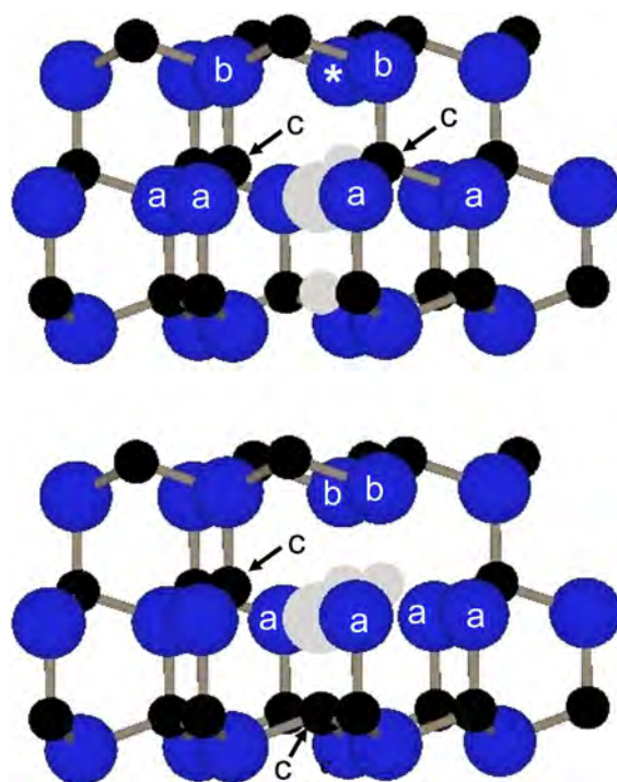
FIG. 8. (Color online) Models showing possible configurations of the trivacancy. The model on top with the two carbon vacancies in a \{1100\} plane is preferred over the one on the bottom with the two vacancies in the basal plane as discussed in the text. The larger balls represent Si atoms and the smaller ones C atoms with light gray balls representing the vacancies. The (a) Si atoms have the 4.2 MHz hyperfine interaction, the (b) Si atoms have the 15.4 MHz hyperfine interaction, and the two C atoms marked with (c) have the principal ^{13}\text{C} hyperfine interaction. The Si site marked with an asterisk may be the C antisite as discussed in the text.
