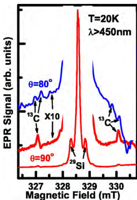
FIG. 7. (Color online) The ^{13}\text{C} hyperfine interaction satellites around the low field EPR line of the ANN1. The angles are with respect to the C axis. The \theta=80^\circ spectrum has been shifted by about 1.15 mT so that the central portions of the spectrum are approximately aligned. (Only the 15.4 MHz ^{29}\text{Si} hyperfine lines are resolved, the 4.2 MHz lines are obscured by the central line.)
