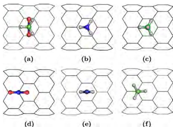
FIG. 3. (Color online) The lowest-energy configurations for simple molecules adsorbed on SWNT(8,0): (a) \text{CH}_3\text{NO}_2 near the hollow site, (b) \text{NH}_3 near the hollow site, (c) \text{CH}_4 near the hollow site, (d) \text{NO}_2 near the top site, (e) \text{NH}_2 near the hollow site, and (f) \text{CH}_3 near the top site.
