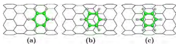
FIG. 1. (Color online) Orientations of C_6H_6 adsorbed on SWNT(8,0): (a) hollow, (b) top, and (c) bridge.
