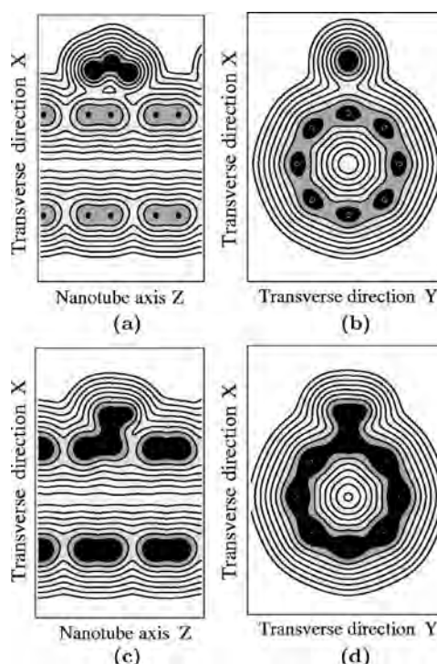
FIG. 7. Total charge-density plots for [(a) and (b)] NO_2/SWNT(8,0) and [(c) and (d)] CH_3/SWNT(8,0) . The contour plots are on a logarithmic scale. In each figure the areas with the largest density are represented by dark gray. (a) and (c) show plots for the SWNT axial cuts; (b) and (d) show plots for cuts perpendicular to the SWNT axis through the functional atoms N and C.
