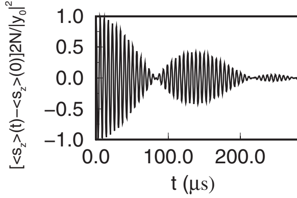
FIG. 2. The time dependence of \langle s_z \rangle from Eq. (16) for the fully polarized case with hyperfine coupling A=90 \mu\text{eV} and \epsilon=A .
