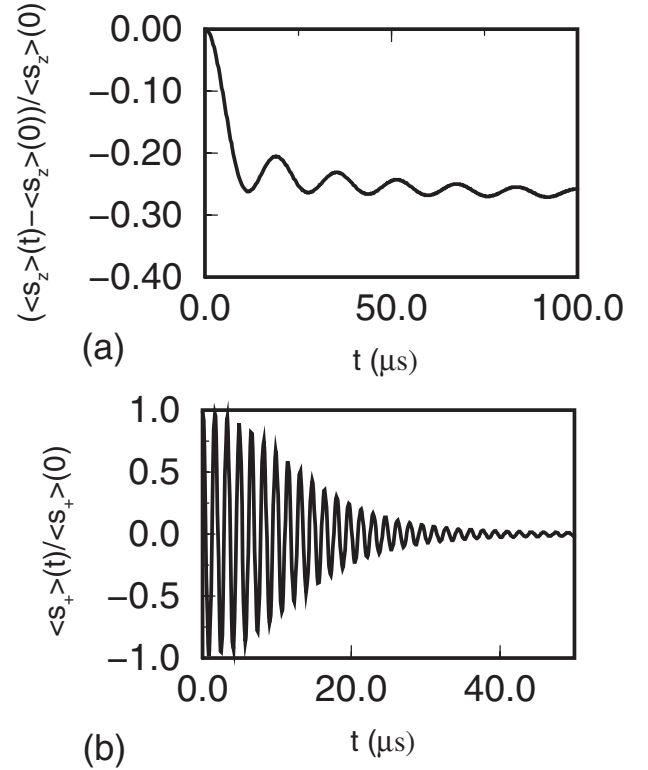
FIG. 1. (a) The time dependence of \langle s_z \rangle from Eq. (13) for initial nuclear polarization of 75% is shown. (b) The time dependence of \langle s_+ \rangle from Eq. (14) for initial nuclear polarization of 75% is shown. We take A = 90 \mu\text{eV} (GaAs) and \epsilon = A .
