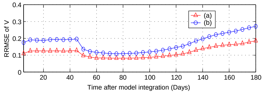
Fig. 7. Temporal evolution of level independent RRMSE due to uncertain winds with the symbol 'Δ' denoting 0.5 m/s noise intensity and the symbol '○' representing 1.0 m/s noise intensity. Note that the error oscillates with an evident error-growing trend.
