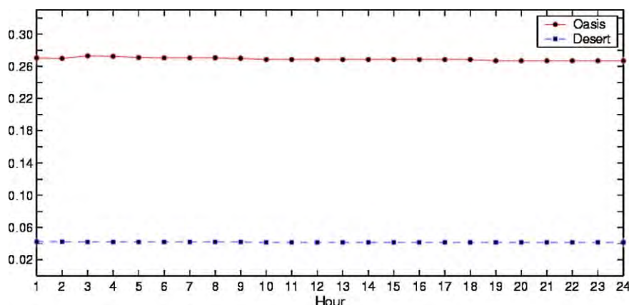
Fig. 7. Simulated temporal variation of total soil moisture (0–2 m) for oasis and desert, showing a stable soil-hydrologic environment.
