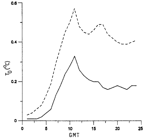
Fig. 18. Subtraction of land-surface temperature ( ^\circ\text{C} ) of medium-oasis from large-oasis (solid) and of small-oasis from large-oasis (dashed) simulation.
