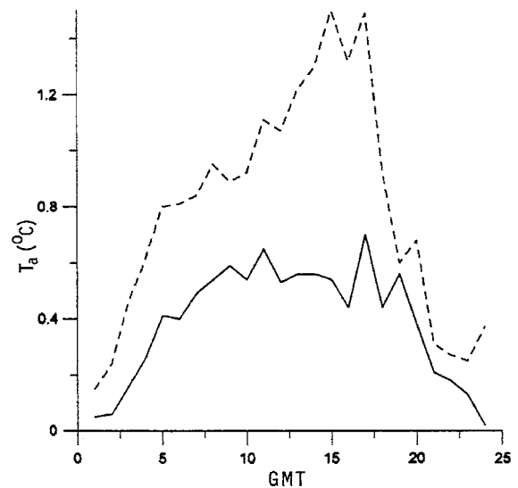
Fig. 19. Subtraction of surface air temperature ( ^\circ\text{C} ) of medium-oasis from large-oasis (solid) and of small-oasis from large-oasis (dashed) simulation.
