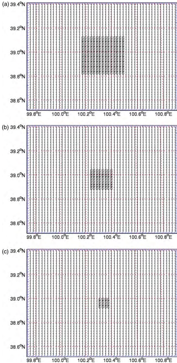
Fig. 17. Three oases in the smallest grid system for numerical investigation: (a) large size with 30\text{ km} \times 30\text{ km} , (b) medium size with 15\text{ km} \times 15\text{ km} , and (c) small size with 7.5\text{ km} \times 7.5\text{ km} . Here, the numbers '6' and '1' denote the oasis and desert, respectively.
