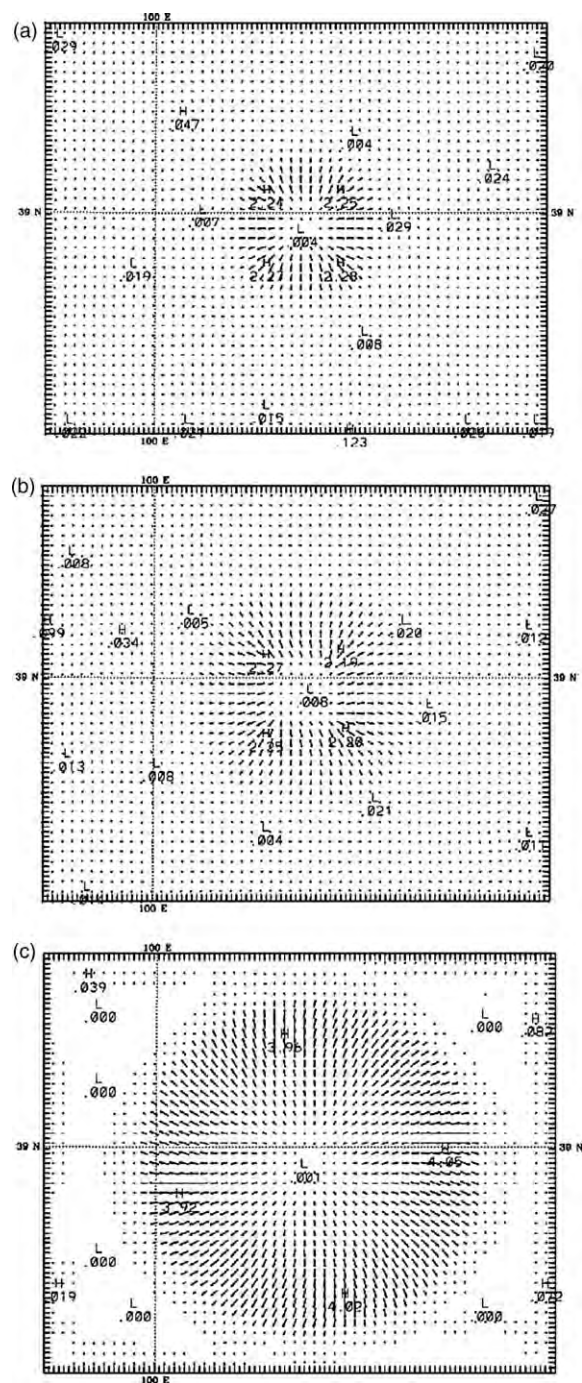
Fig. 12. Simulated surface (850 hPa) wind vector field at (a) 0600 GMT (1300 LT), (b) 0900 GMT (1600 LT), and (c) 1200 GMT (1900 LT).
