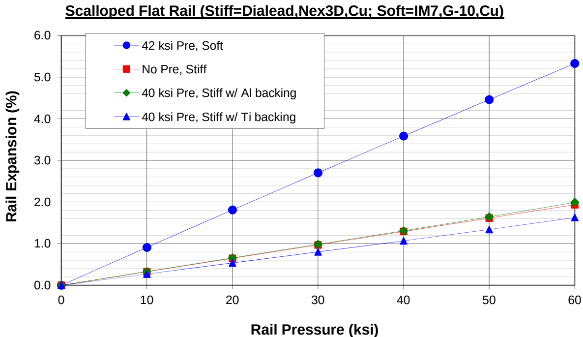
Figure 16. Scalloped Flat Rail Design Rail Expansion
