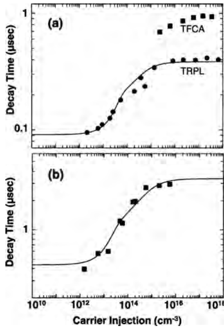
FIG. 1. Injection dependence of the PL decay time for (a) sample A and (b) sample B. The PL decay time is compared in (a) to that determined by TFCA at the same location on the sample. The factor of 2 difference in lifetime expected between these techniques is apparent. The solid lines are the result of carrier dynamics simulations described in Sec. IV.
