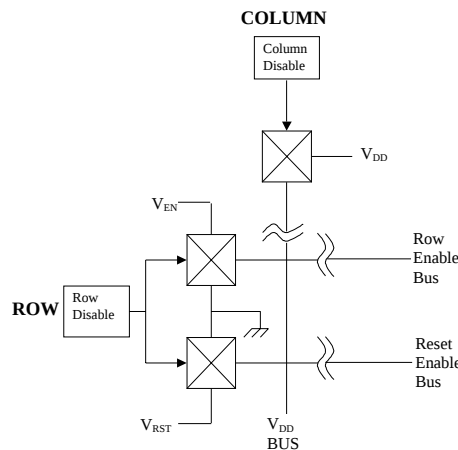
Figure 5. Row and column disable logic block diagram for the Orion II readout
