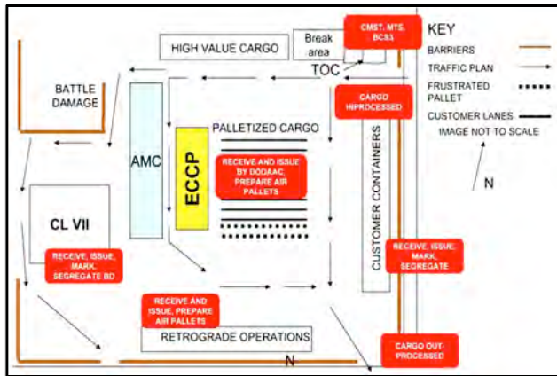
Figure 7: CRSP layout.
