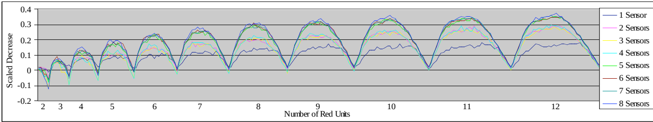
Figure 3: The value of sensor information in terms of the scaled percent decrease in red score.
