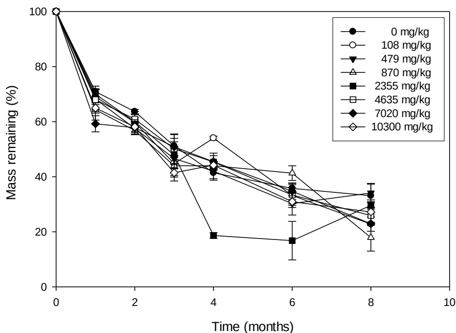
Figure 5. Effect of CL-20 on decomposition of Orchard grass ( Dactylis glomerata ) litter in Sassafras sandy loam soil.
