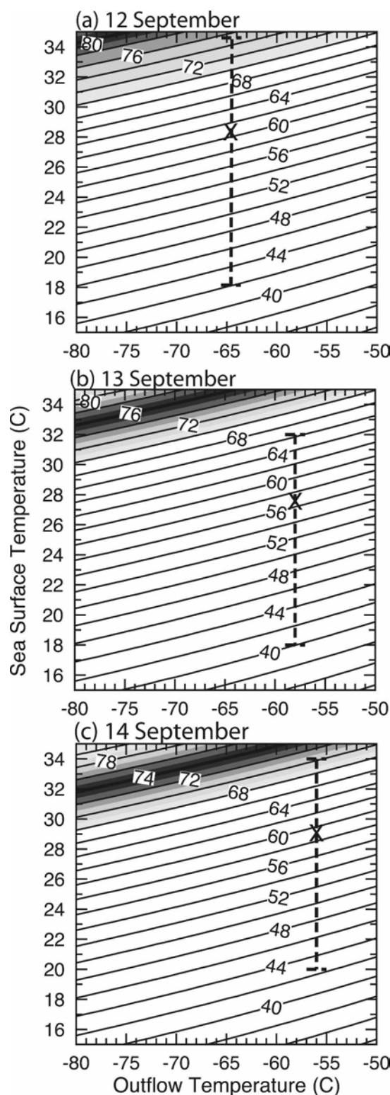
FIG. 13. Theoretically predicted azimuthal mean V_{\max} at the boundary layer top for varying outflow temperature and near-core SST with a constant RH = 80\% . The “X” indicates the primary potential intensity estimate for the observed near environment around Isabel. The dark solid curve represents the av-
