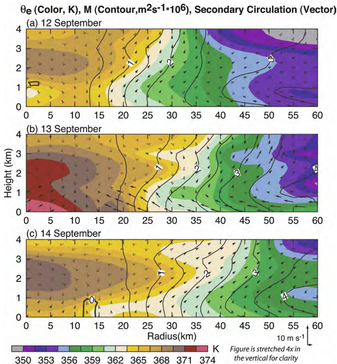
FIG. 5. Radius–height azimuthal mean storm-relative \theta_e (color; K); absolute angular momentum (contour; \text{m}^2 \text{s}^{-1} \times 10^6 ); and transverse secondary circulation (vector) from (a) 12, (b) 13, and (c) 14 Sep 2003.
