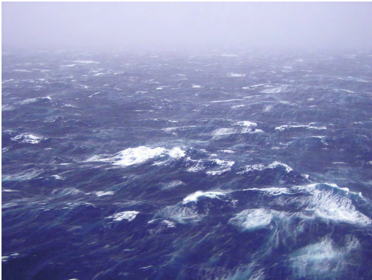
FIG. 12. Photograph of sea surface in Hurricane Isabel taken from NOAA 43 during stepped descent pattern below 400-m altitude. Surface wind speed is 20\text{--}30\text{ m s}^{-1} . (Photo courtesy of M. Black.)
