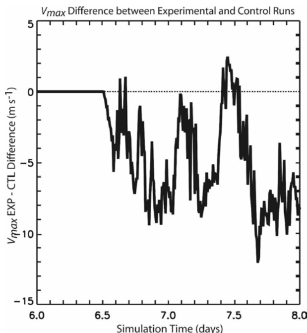
FIG. A1. Difference in the maximum tangential wind ( V_{\max} ) between the experimental run (EXP) and control run (CTL) over time of the axisymmetric hurricane model described in PM03 and Rotunno and Emanuel (1987). The EXP run imposes 1°C SST reduction underneath the eyewall at 6.5 days into the simulation to mimic the passage over a cool hurricane wake.
