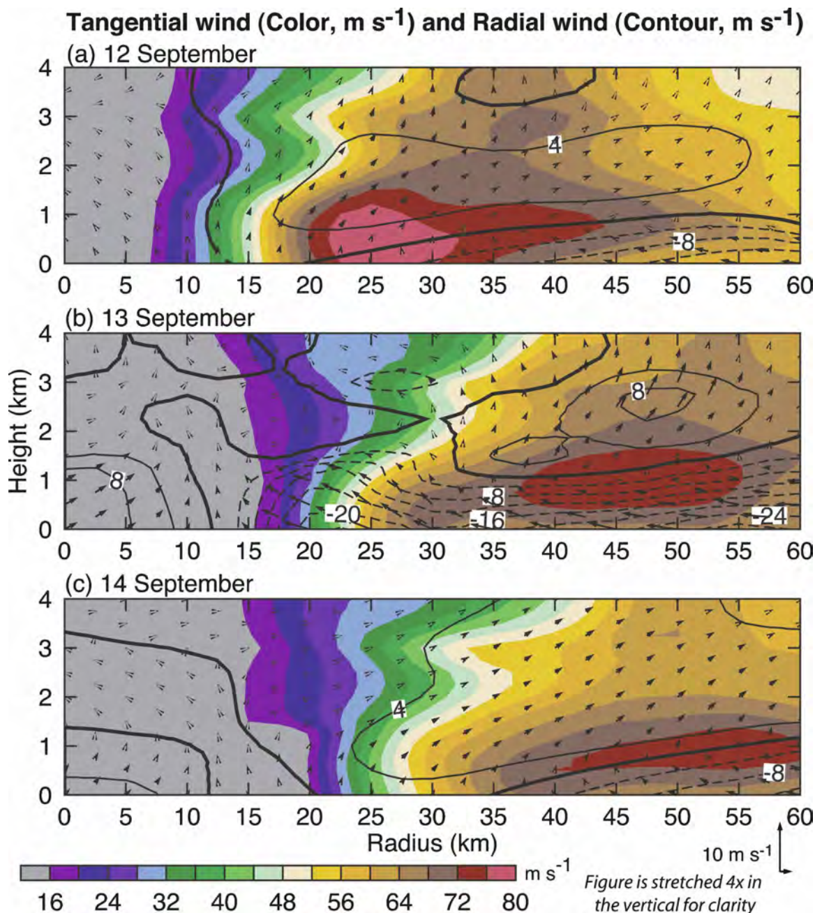
FIG. 4. Radius–height azimuthal mean storm-relative tangential wind (color), radial wind (contour), and the secondary circulation (vector) in \text{m s}^{-1} derived from GPS dropwindsonde and flight-level data from (a) 12, (b) 13, and (c) 14 Sep 2003.
