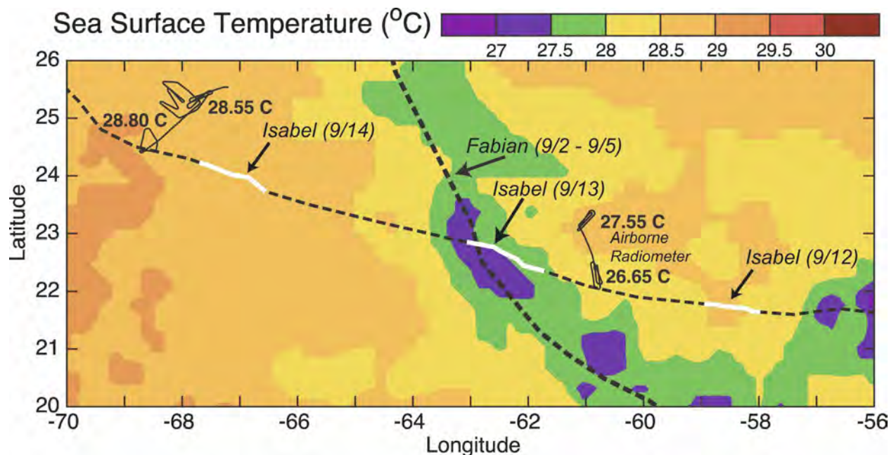
FIG. 10. SST derived from AVHRR satellite (average SST over 4–10 Sep in color) and NOAA WP-3D downward-pointing radiometer (thin line, from ~1800 UTC 13 and 14 Sep). Tracks of Hurricanes Fabian (dashed best track, from 2 to 5 Sep) and Isabel (dashed best track, with thick white, solid line indicating analysis periods from 1600 to 2300 UTC 12–14 Sep) are shown for reference.
